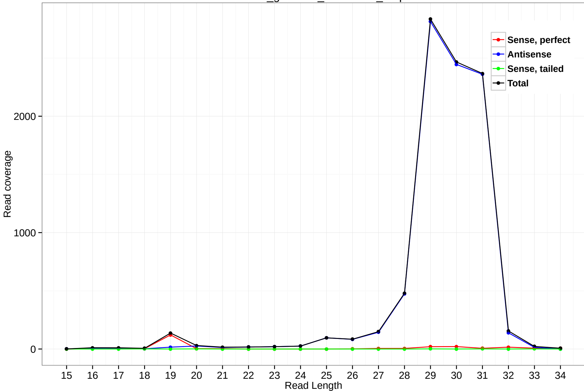
rheMac3_genscan_chr7.1515_5.5p
