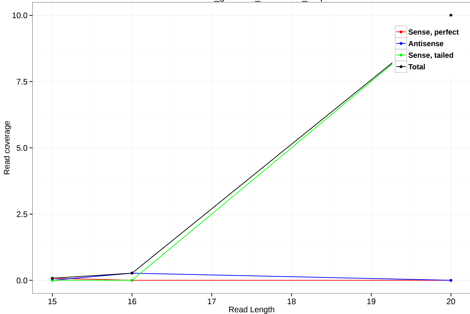
rheMac3_genscan_chr7.1487_0.5p
