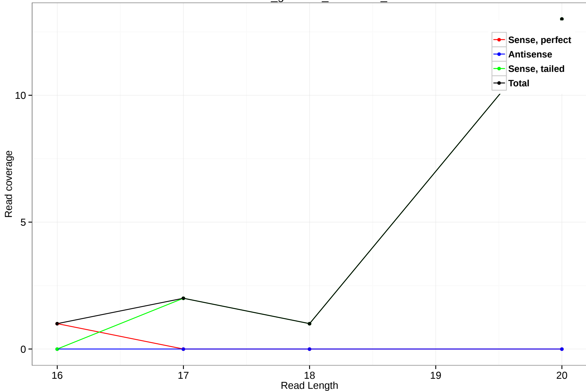
rheMac3_genscan_chr7.1454_5
