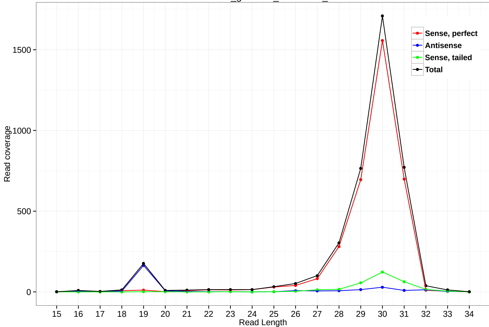
rheMac3_genscan_chr7.1442_1
