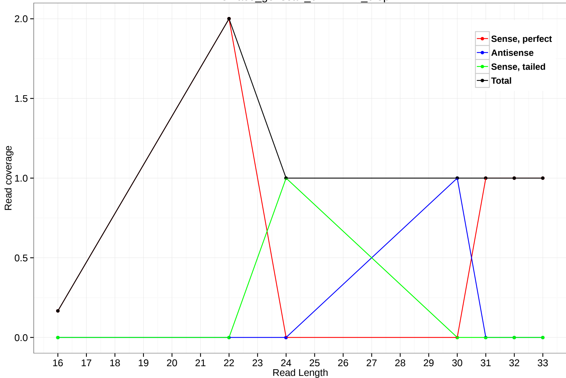
rheMac3_genscan_chr7.1424_0.3p
