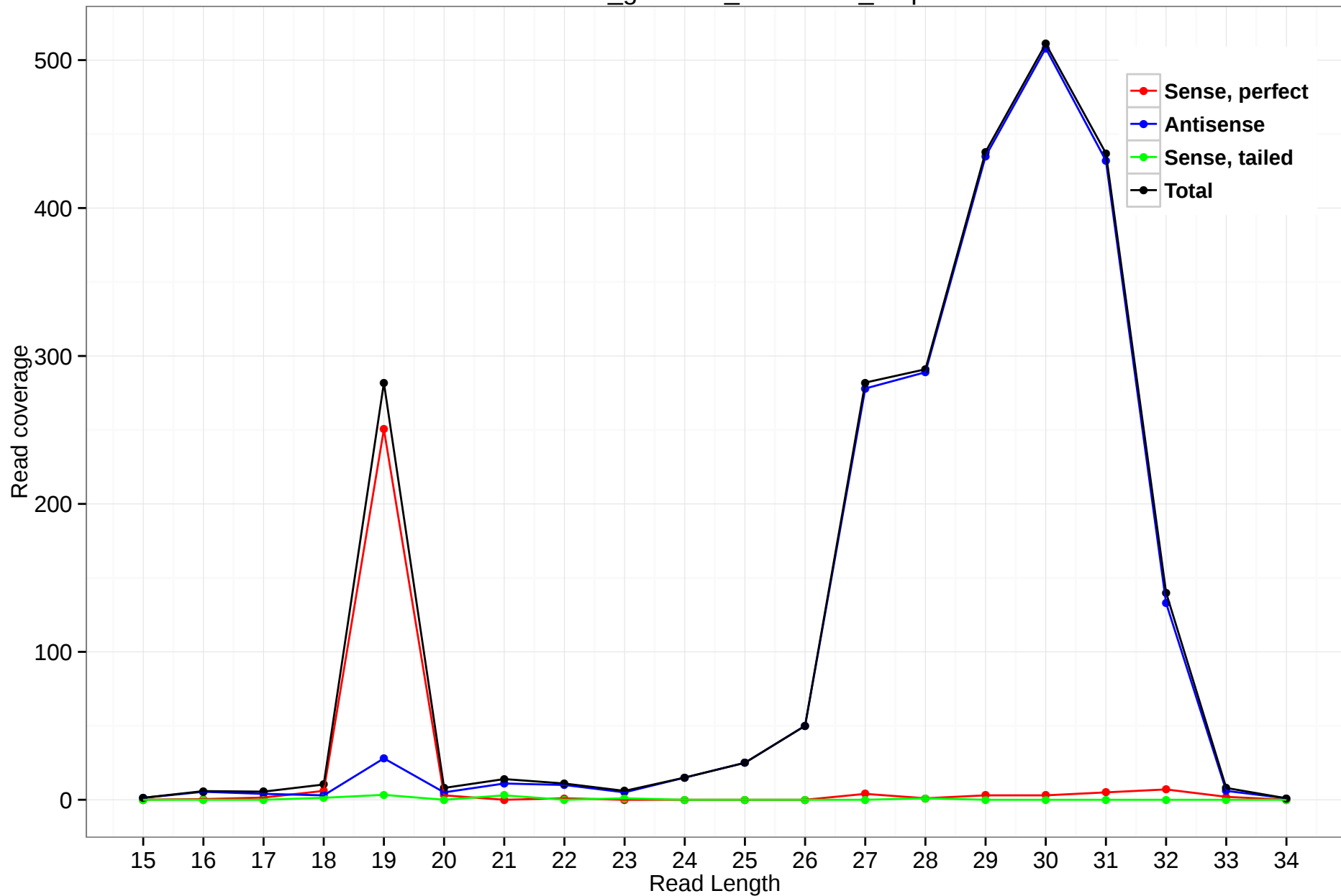
rheMac3_genscan_chr7.1421_7.5p
