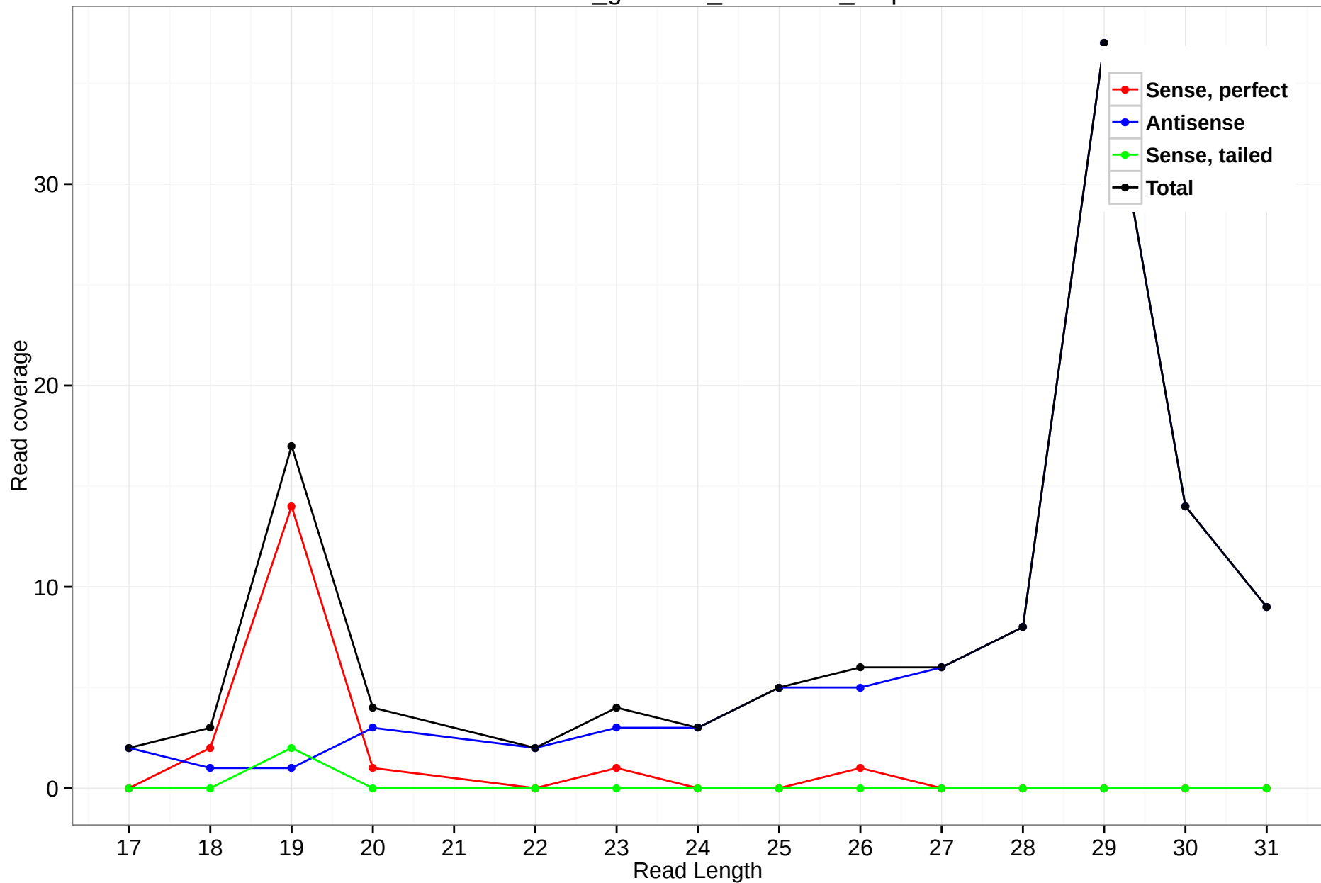
rheMac3_genscan_chr7.1421_4.5p
