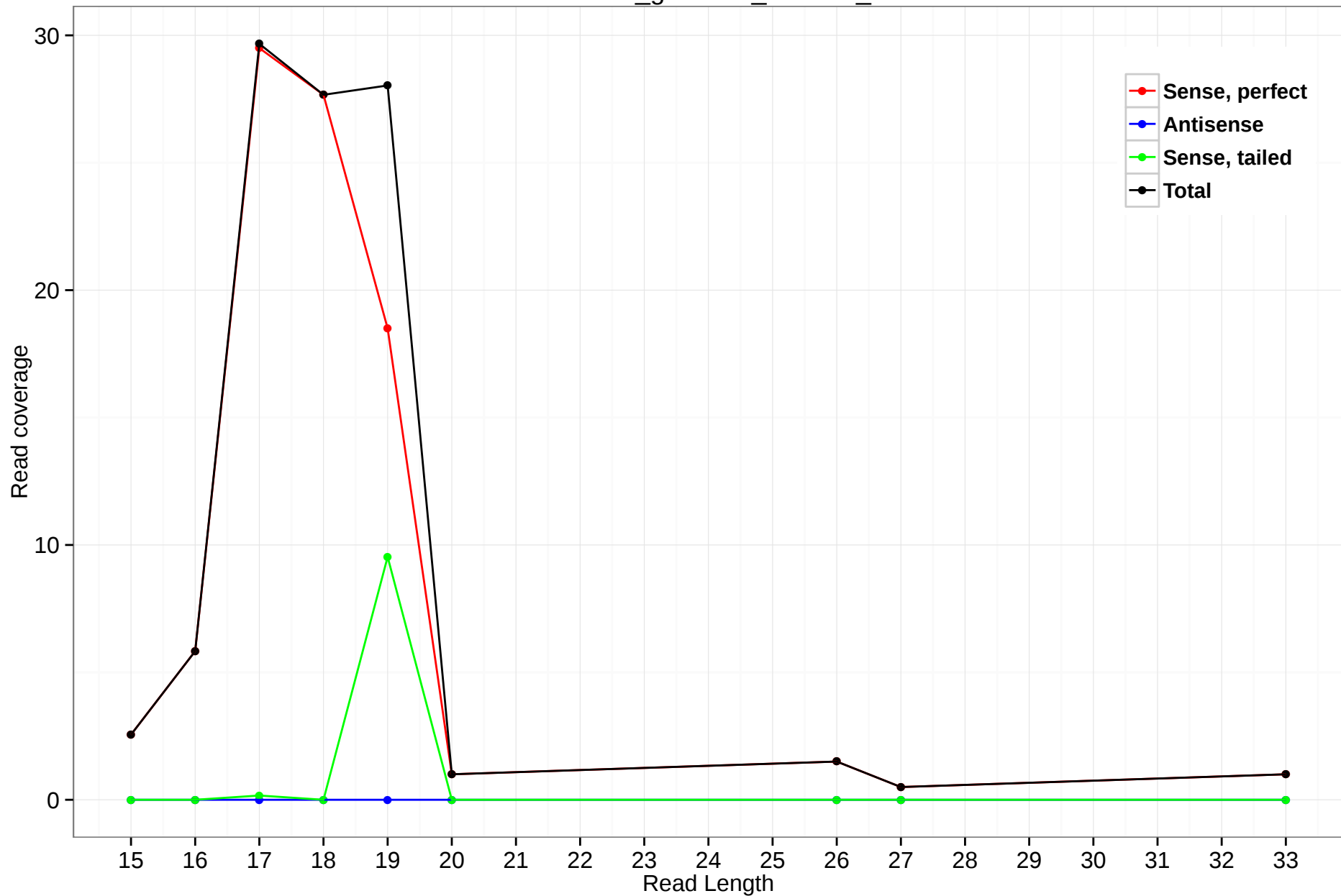
rheMac3_genscan_chr7.13_7
