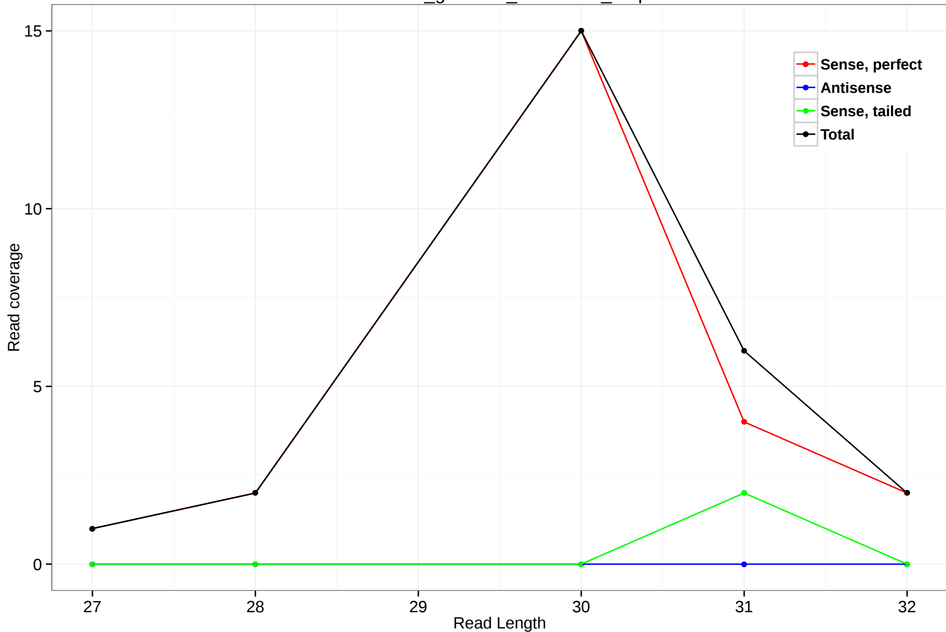
rheMac3_genscan_chr7.1375_6.3p
