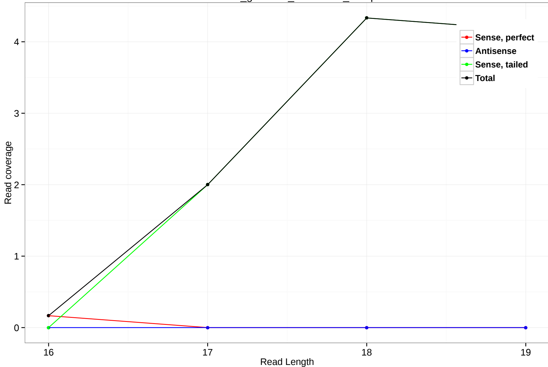
rheMac3_genscan_chr7.1309_12.3p
