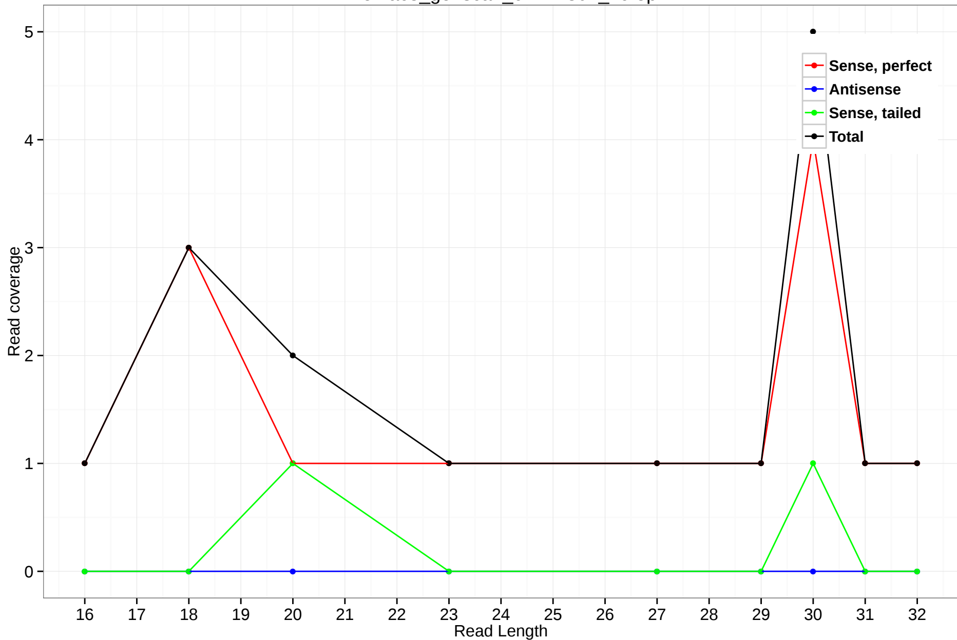
rheMac3_genscan_chr7.1301_29.5p
