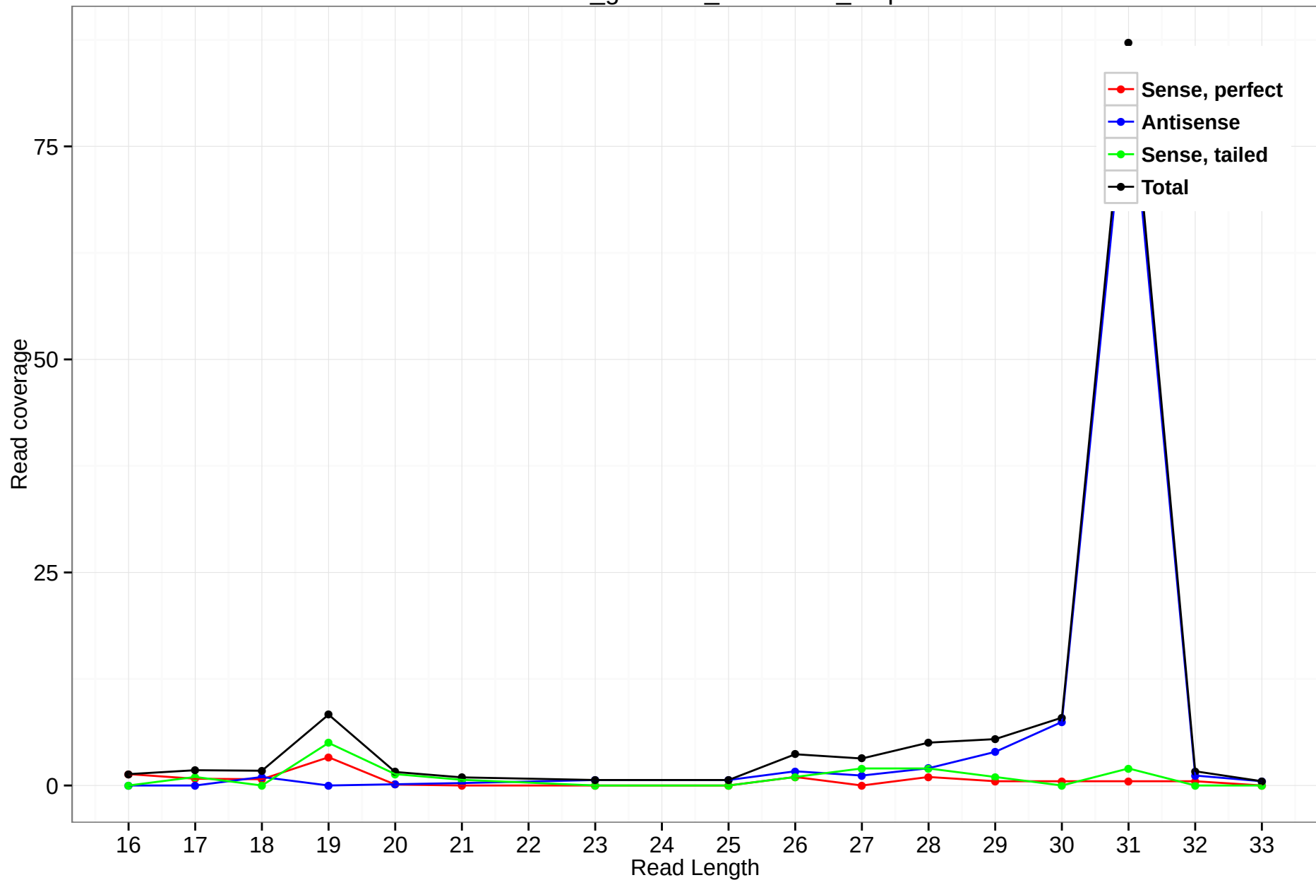
rheMac3_genscan_chr7.1299_1.5p
