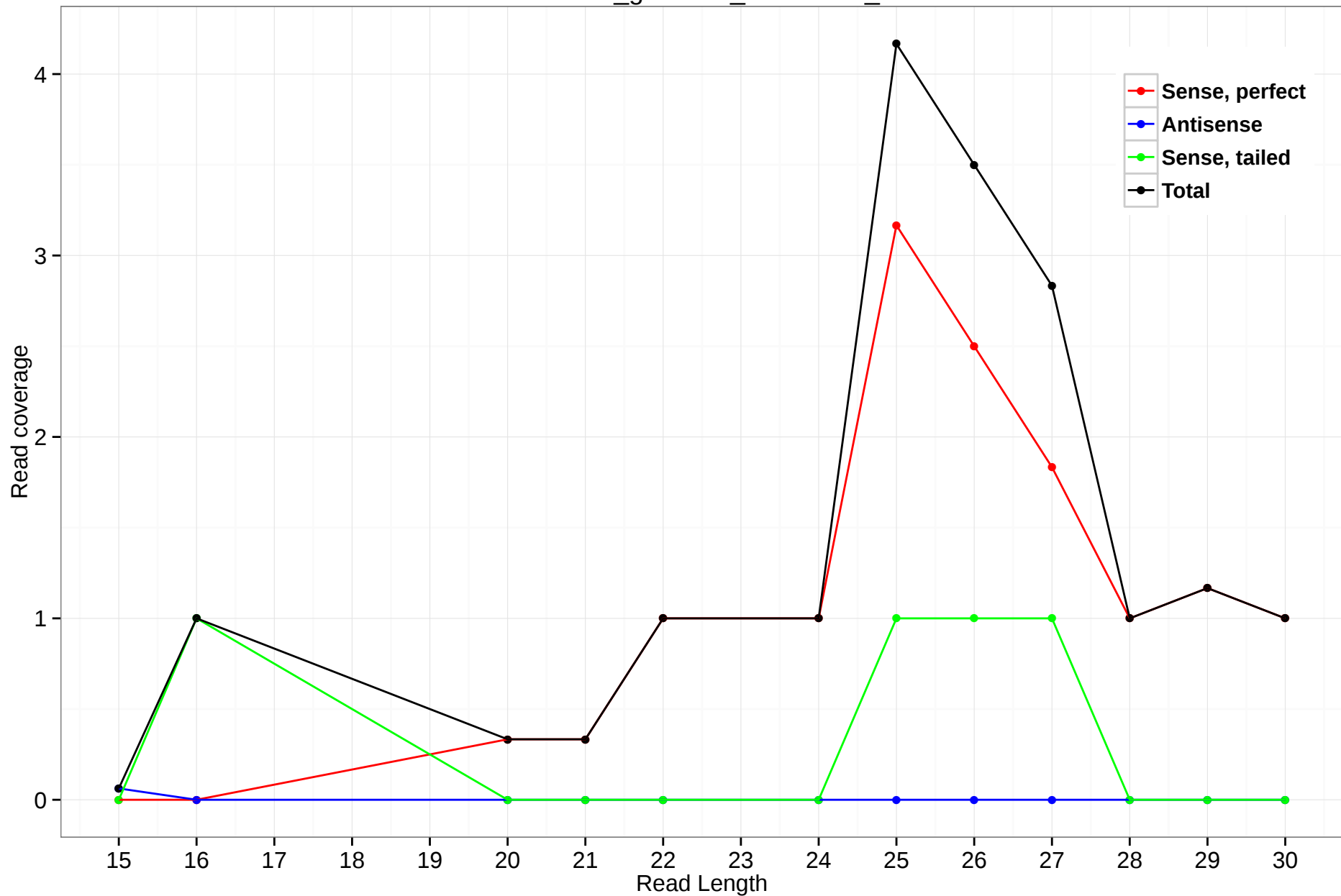
rheMac3_genscan_chr7.1291_3
