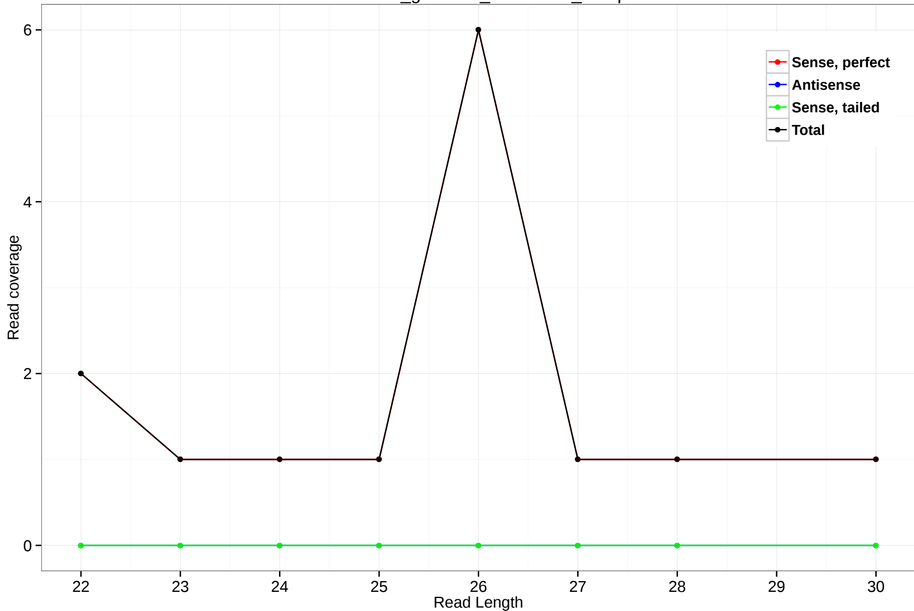
rheMac3_genscan_chr7.1291_17.3p
