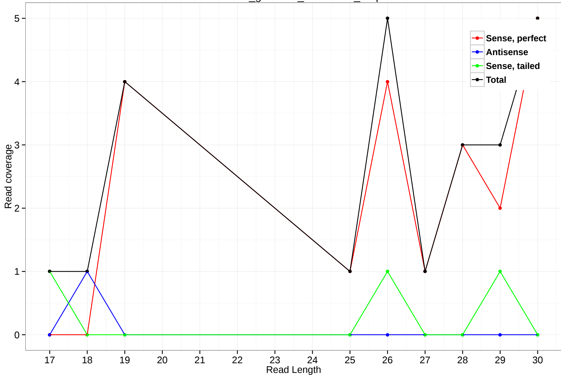
rheMac3_genscan_chr7.1290_2.3p
