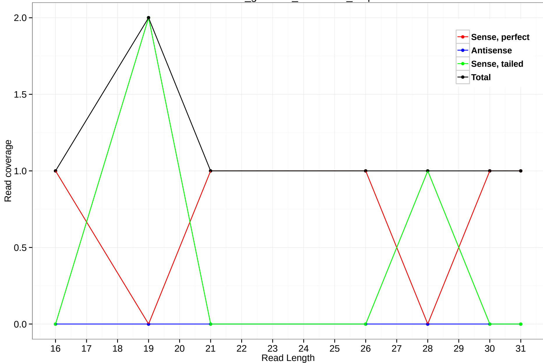
rheMac3_genscan_chr7.1285_3.5p
