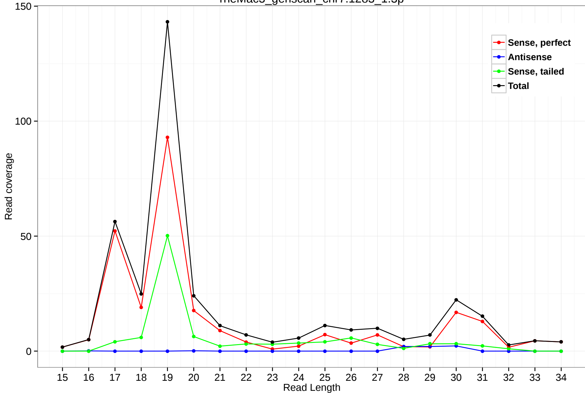
rheMac3_genscan_chr7.1283_1.3p
