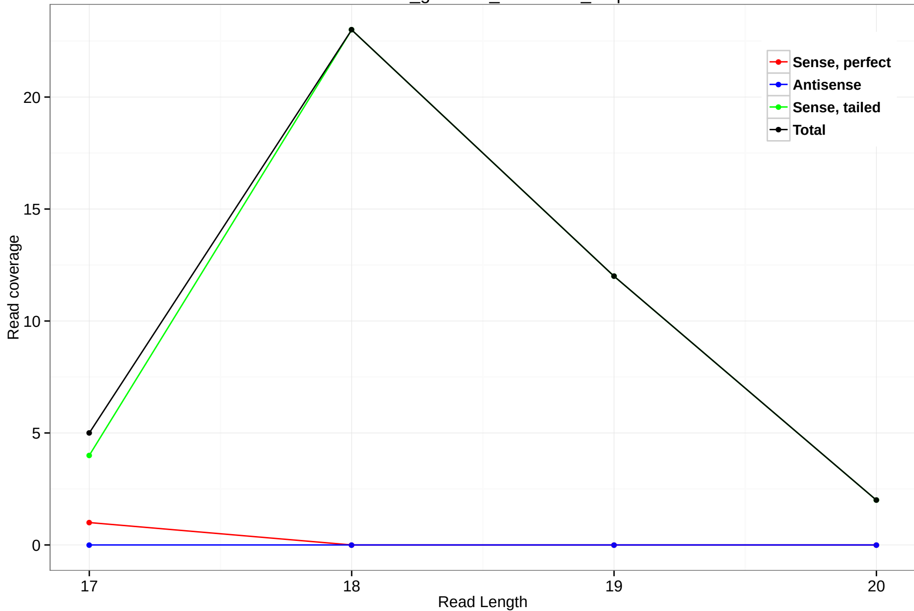
rheMac3_genscan_chr7.1257_0.5p
