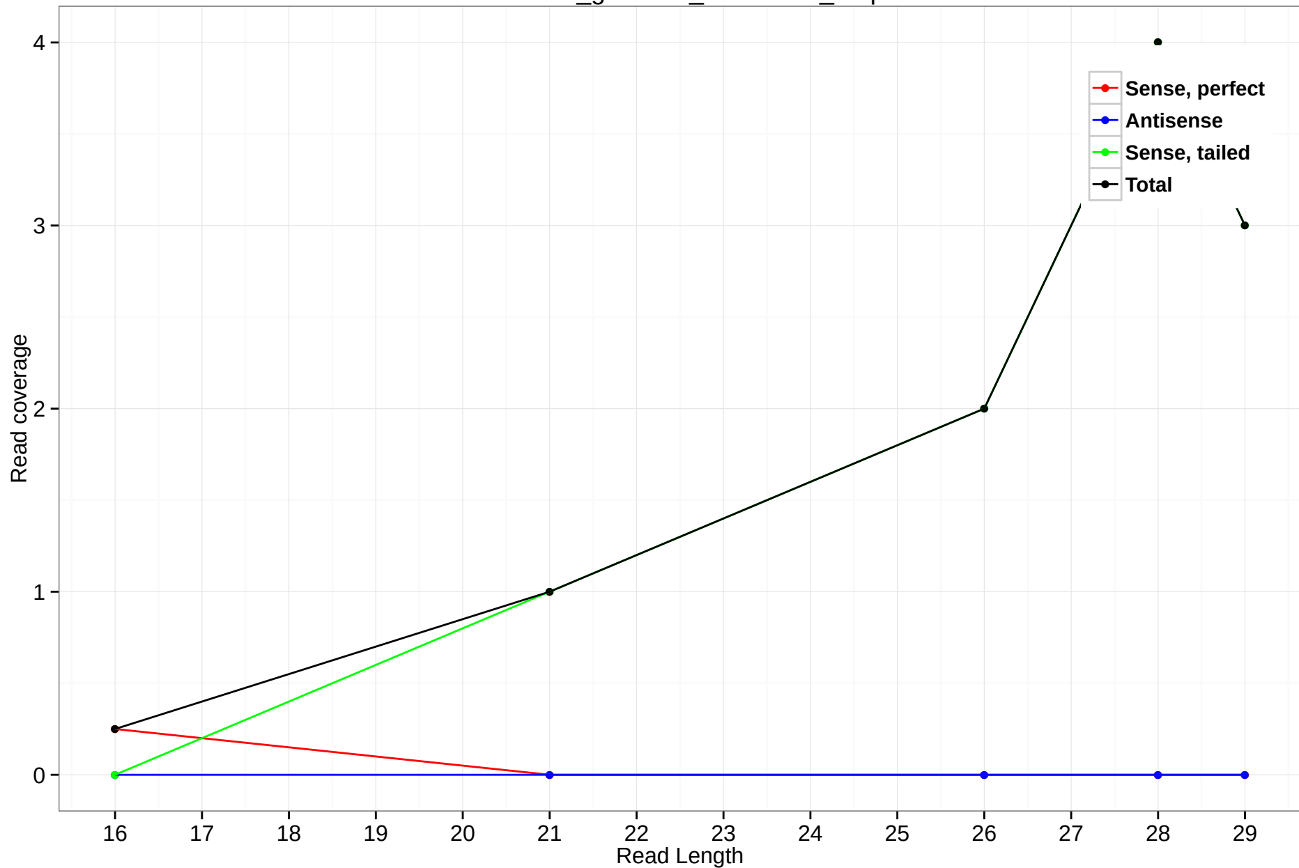
rheMac3_genscan_chr7.1254_9.5p
