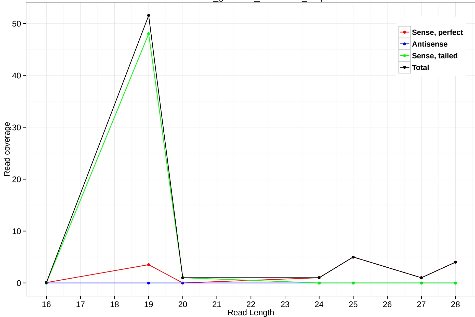
rheMac3_genscan_chr7.1245_5.5p
