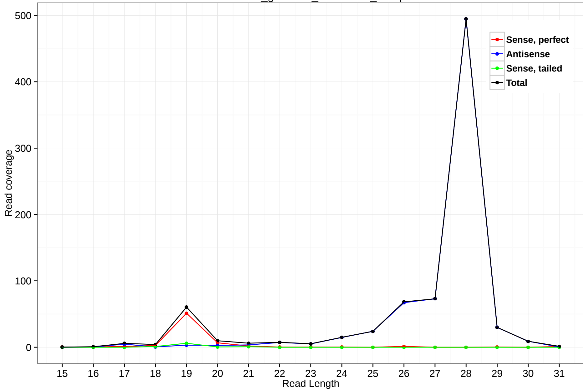
rheMac3_genscan_chr7.1245_11.5p
