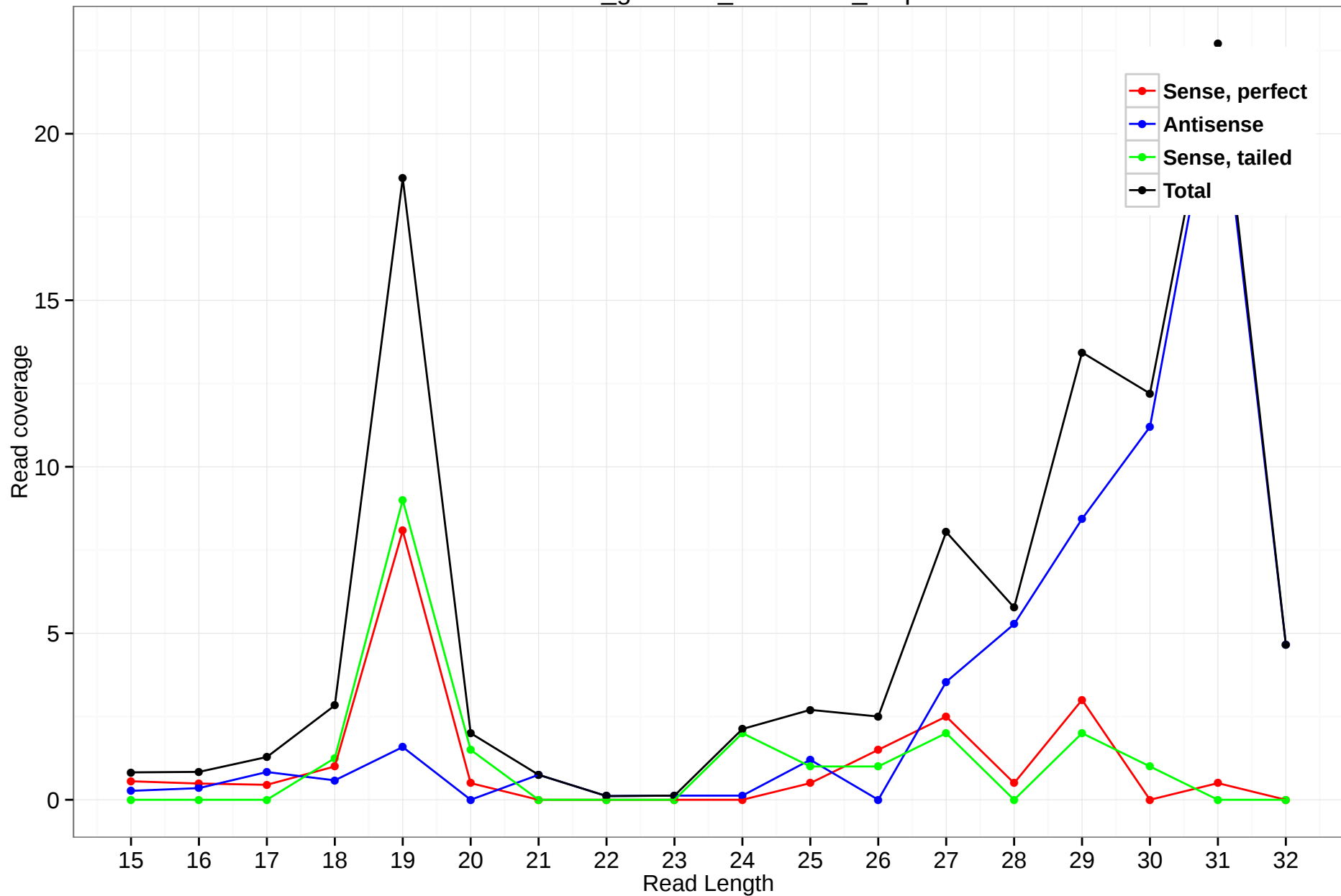
rheMac3_genscan_chr7.1244_6.3p
