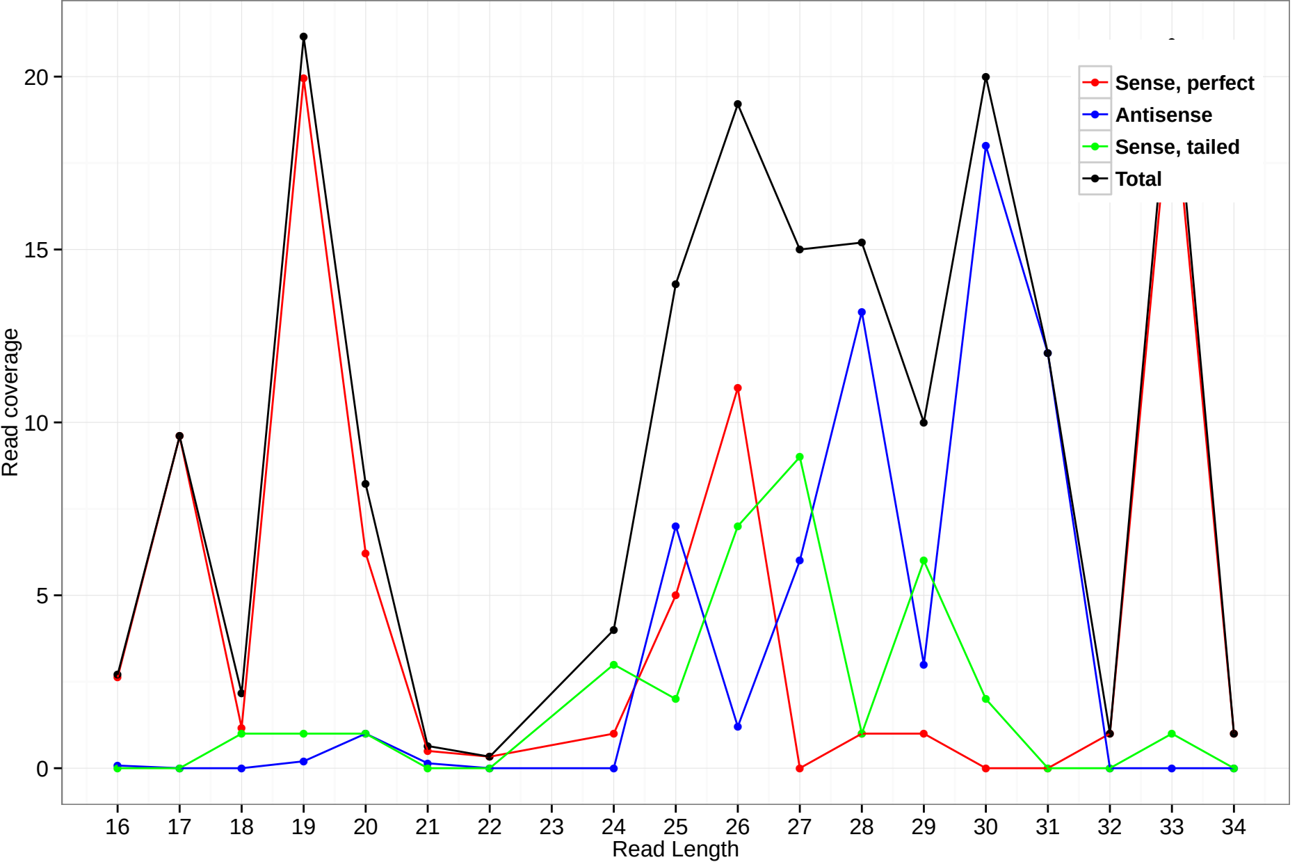
rheMac3_genscan_chr7.1244_10
