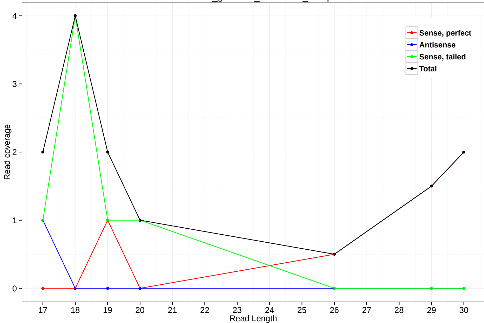
rheMac3_genscan_chr7.1239_21.5p
