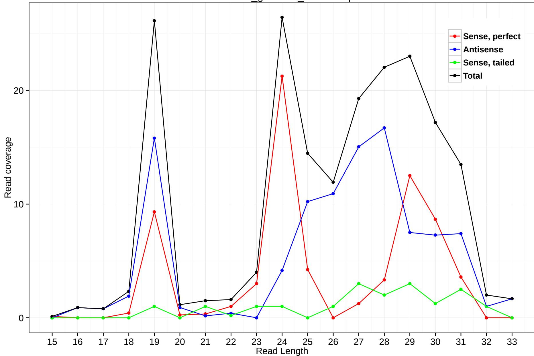
rheMac3_genscan_chr7.12.3p
