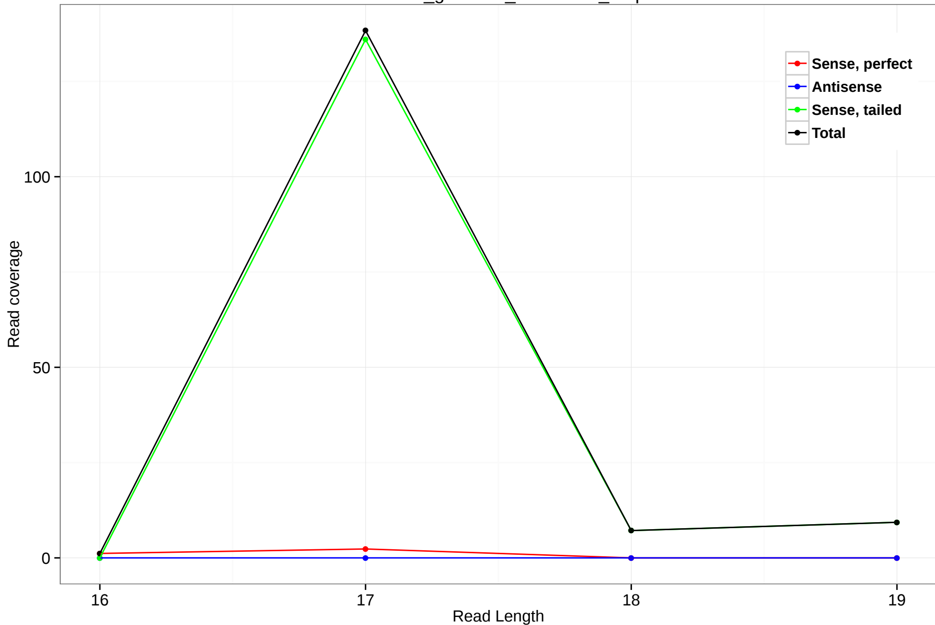
rheMac3_genscan_chr7.1157_2.3p
