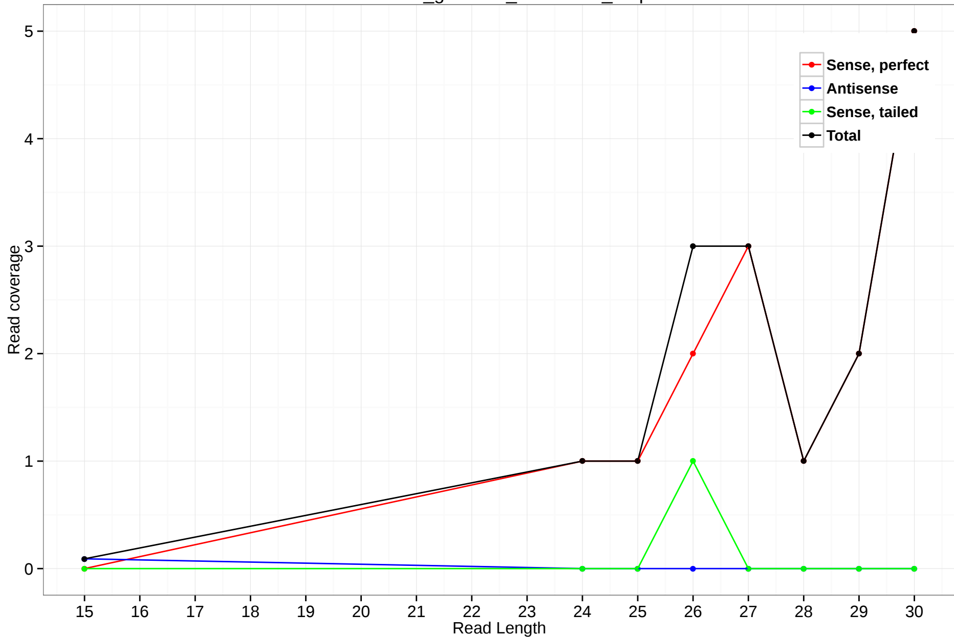
rheMac3_genscan_chr7.1148_6.5p
