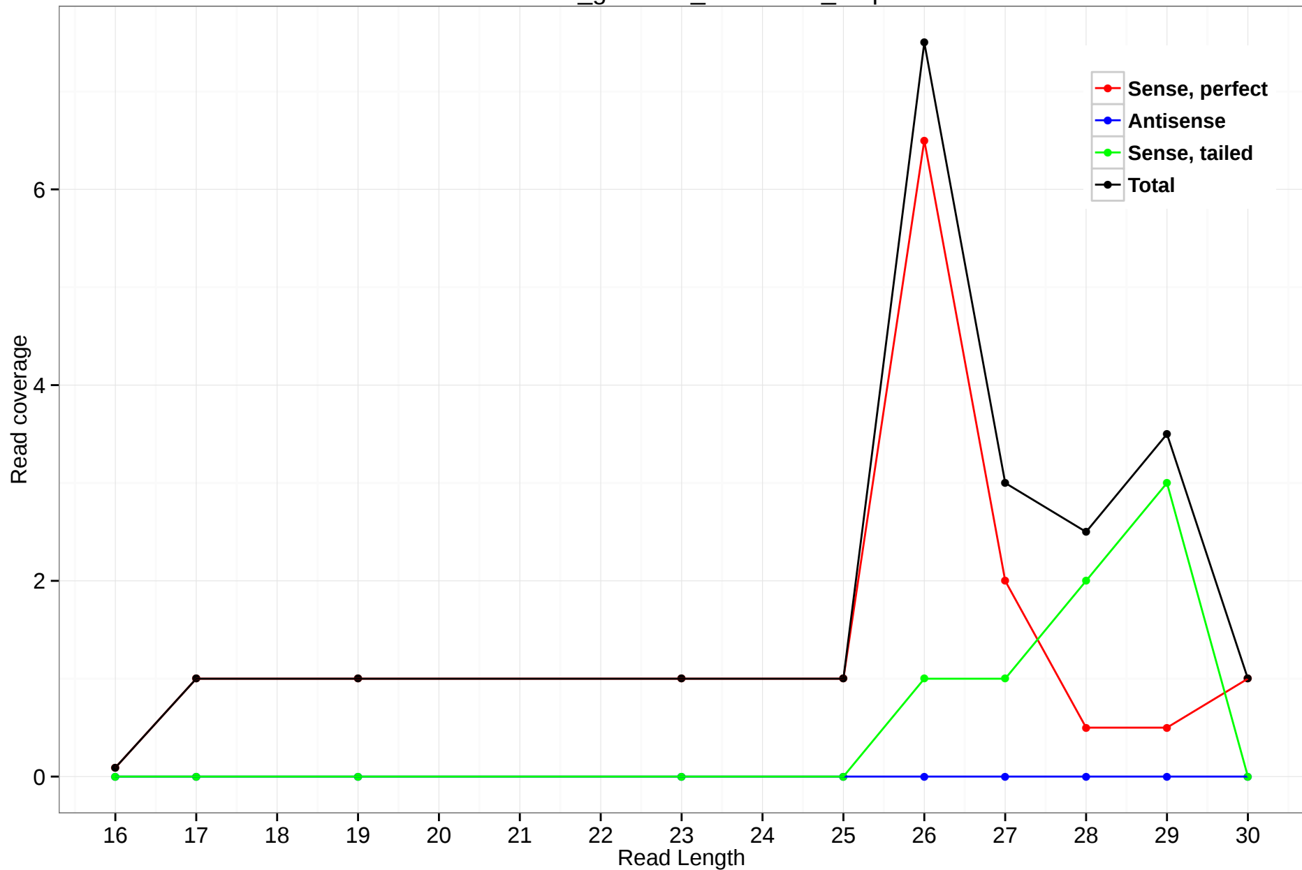
rheMac3_genscan_chr7.1133_2.5p
