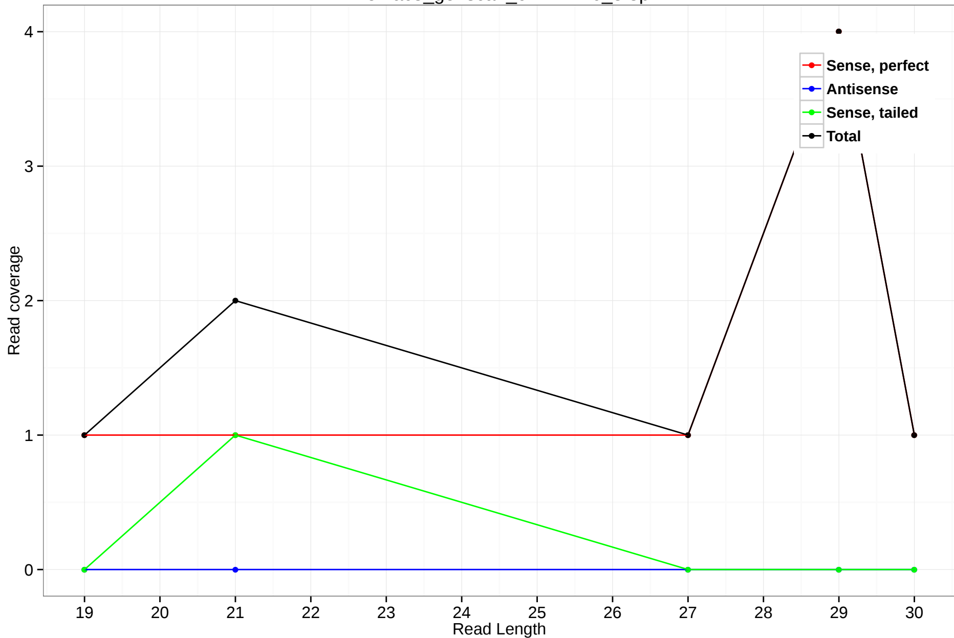
rheMac3_genscan_chr7.1126_3.3p
