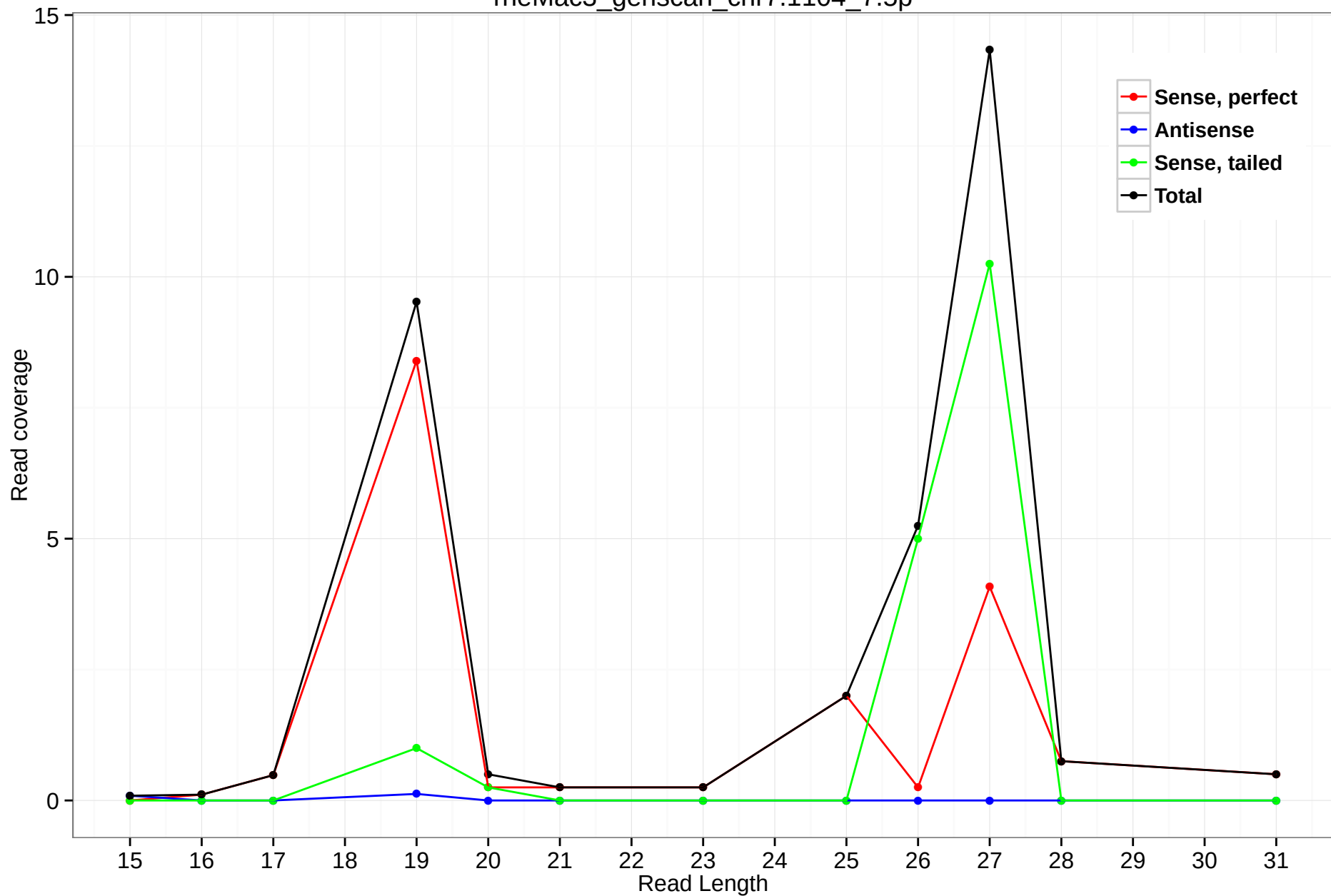
rheMac3_genscan_chr7.1104_7.5p
