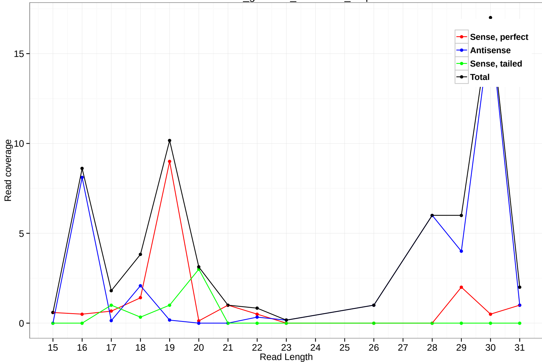
rheMac3_genscan_chr7.1104_1.3p
