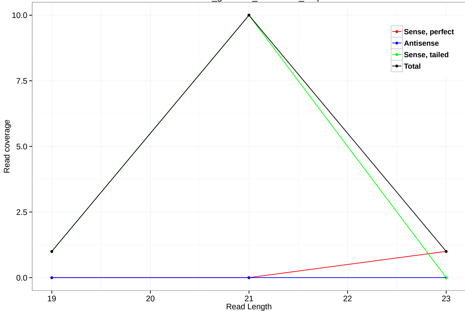
rheMac3_genscan_chr7.1101_1.5p
