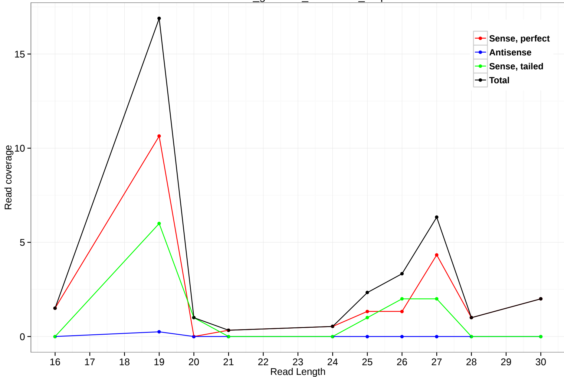
rheMac3_genscan_chr7.1100_2.3p
