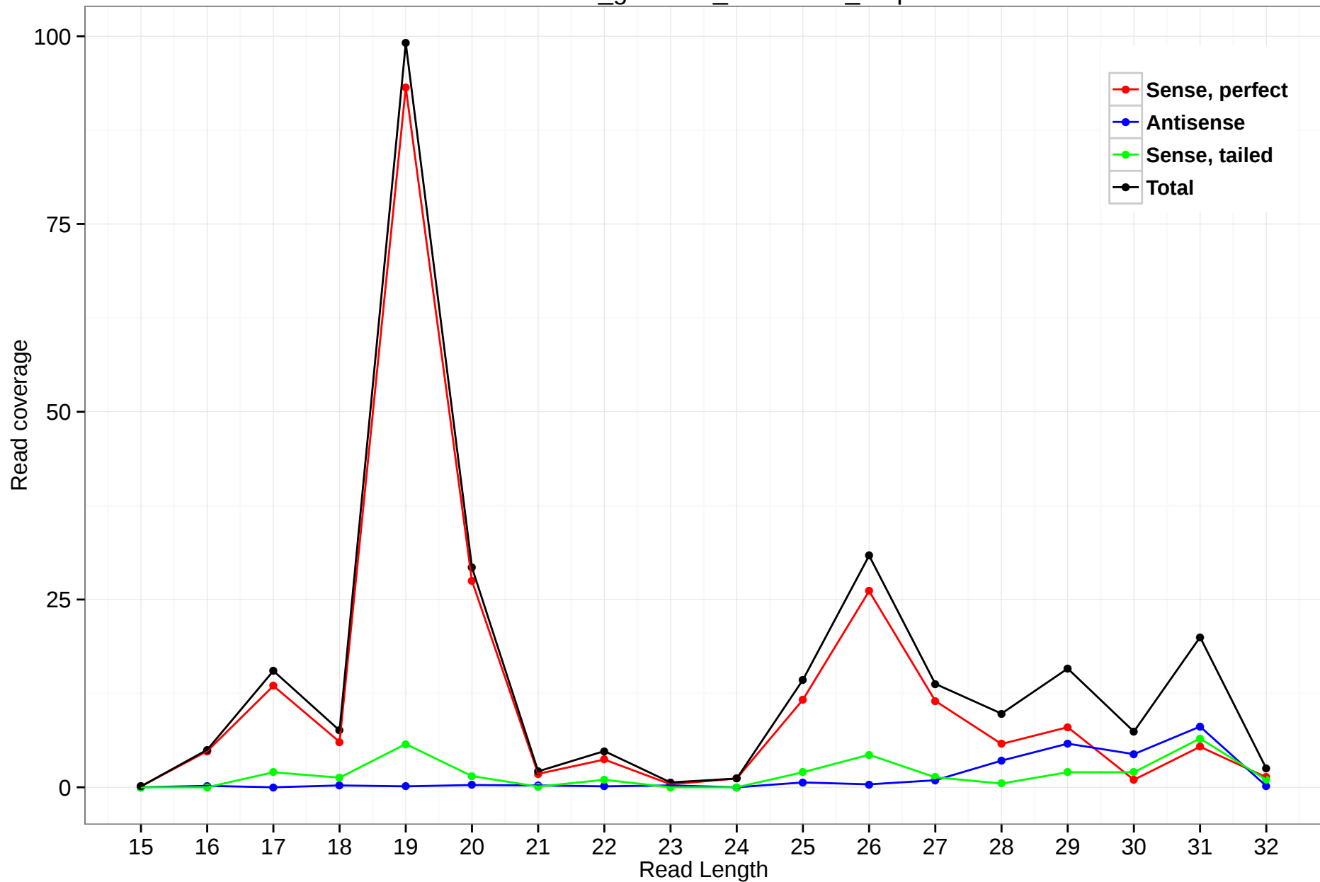
rheMac3_genscan_chr7.1100_1.5p
