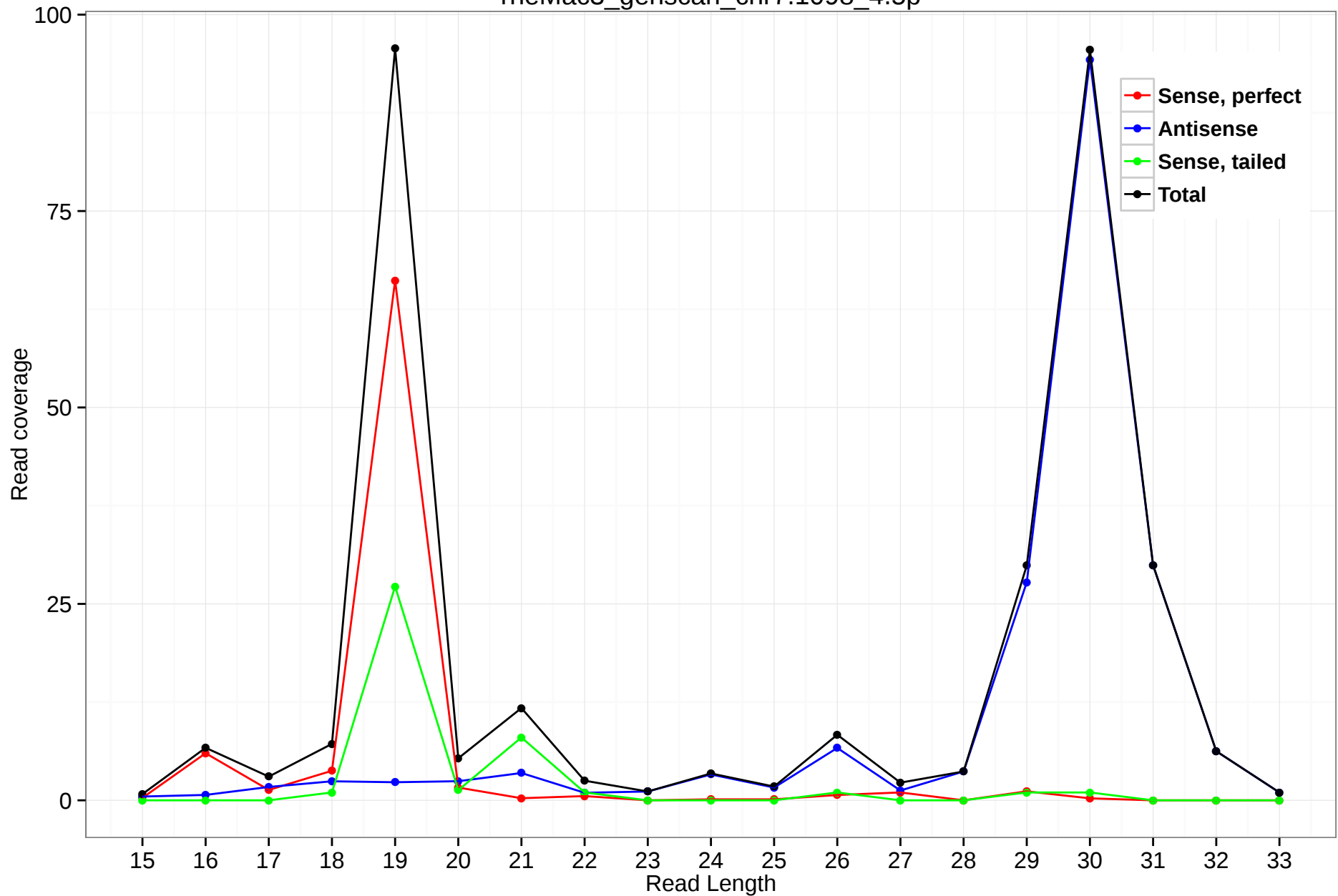
rheMac3_genscan_chr7.1098_4.5p
