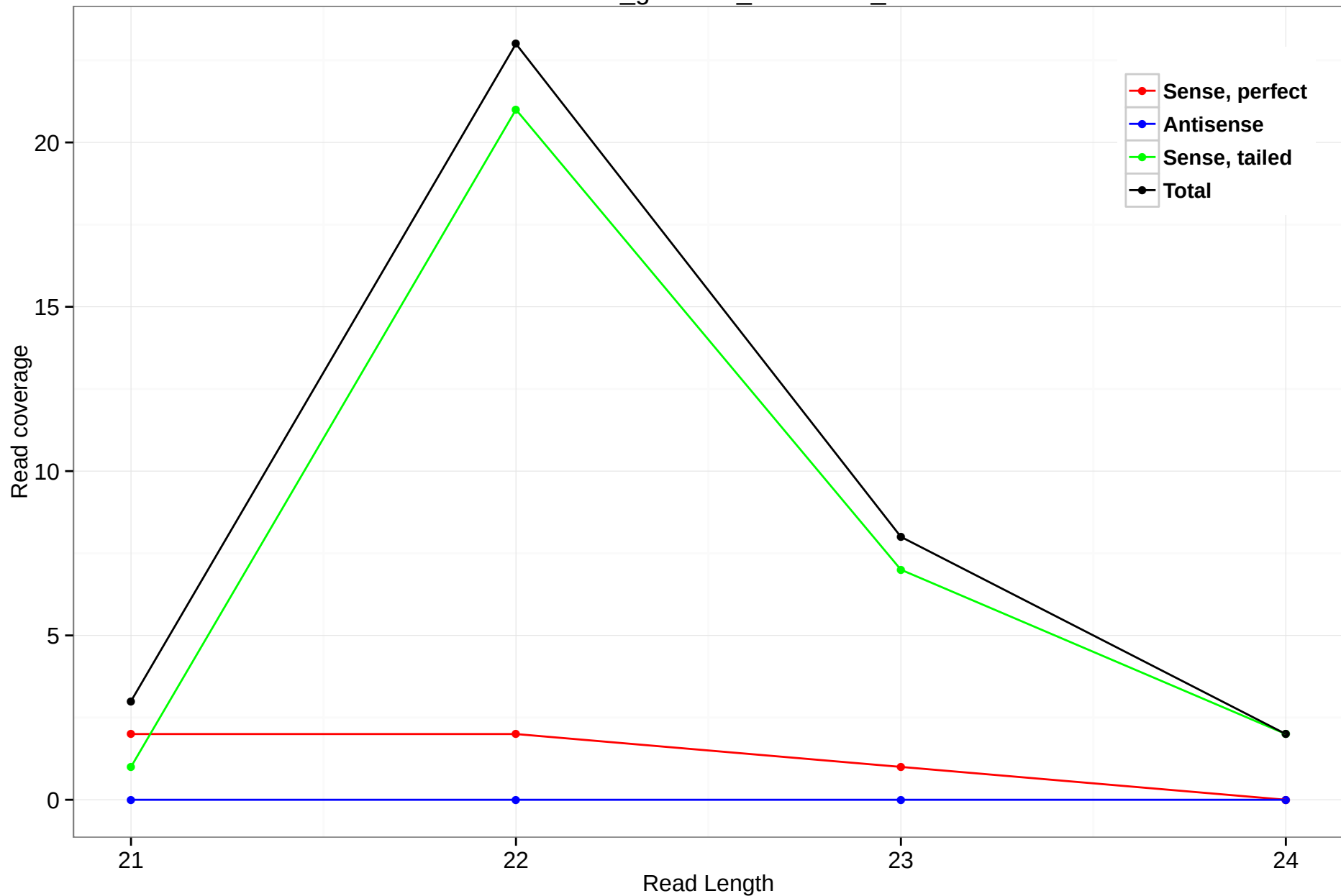
rheMac3_genscan_chr7.1088_5
