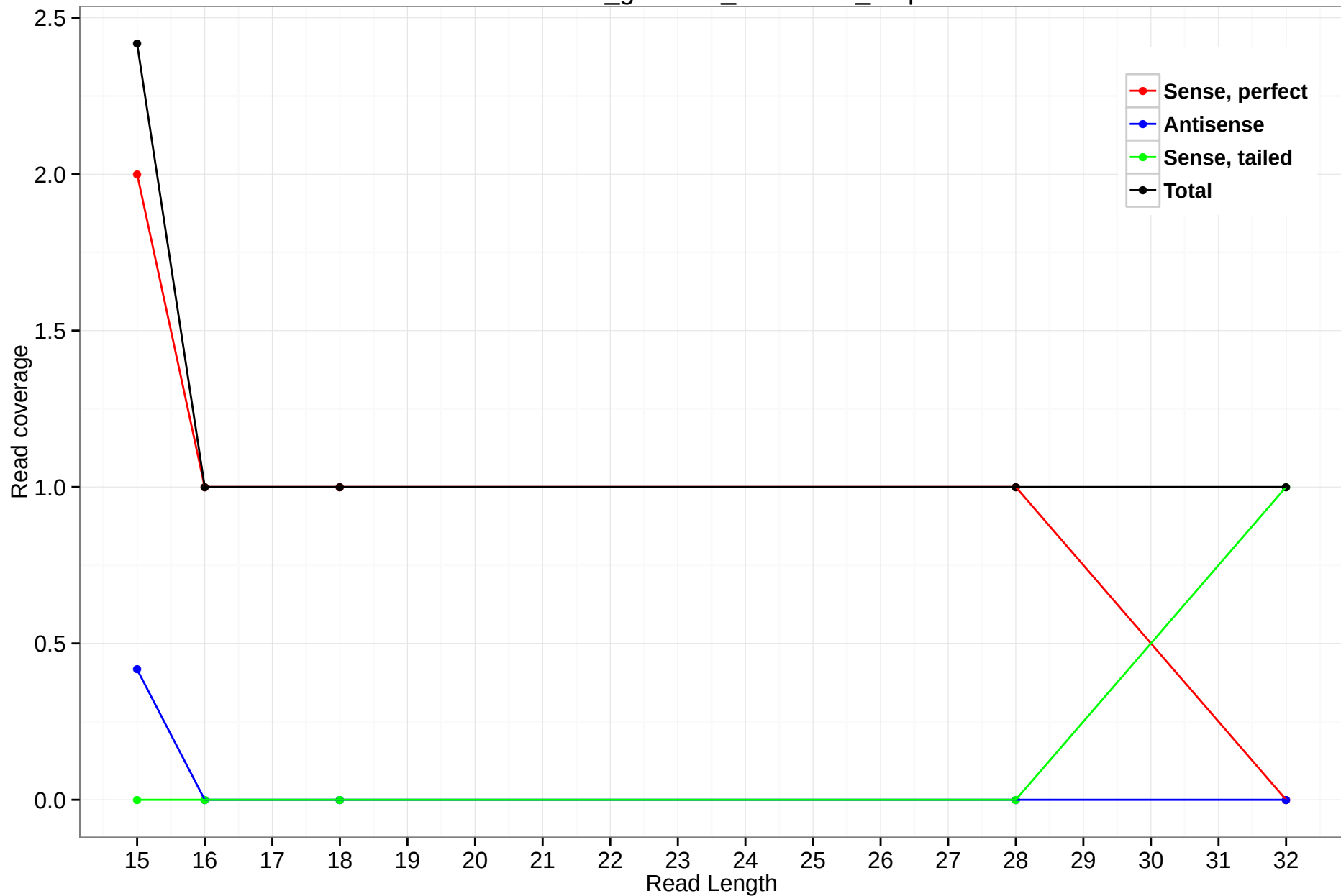
rheMac3_genscan_chr7.1071_0.5p
