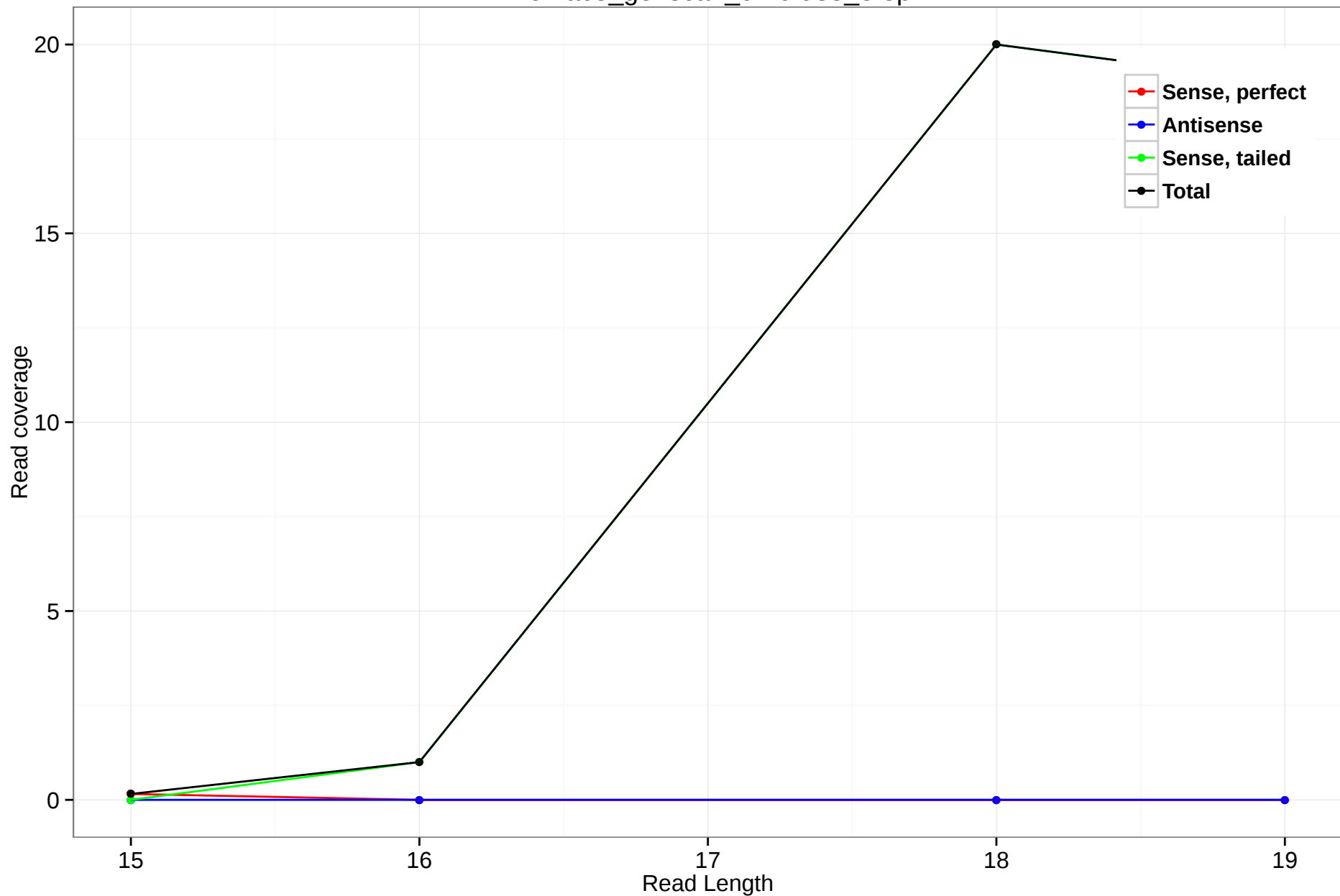
rheMac3_genscan_chr6.933_8.3p
