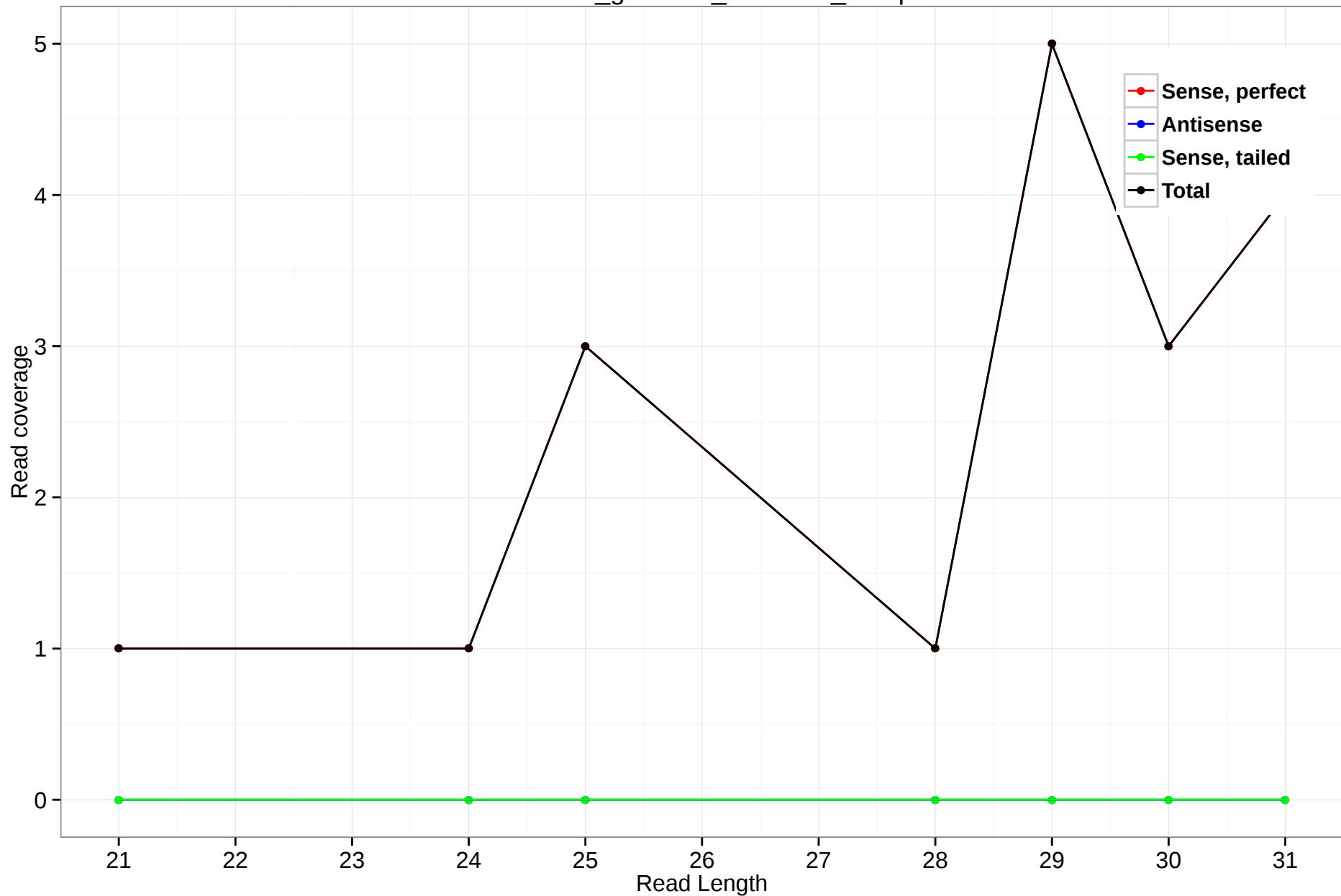
rheMac3_genscan_chr6.926_10.5p
