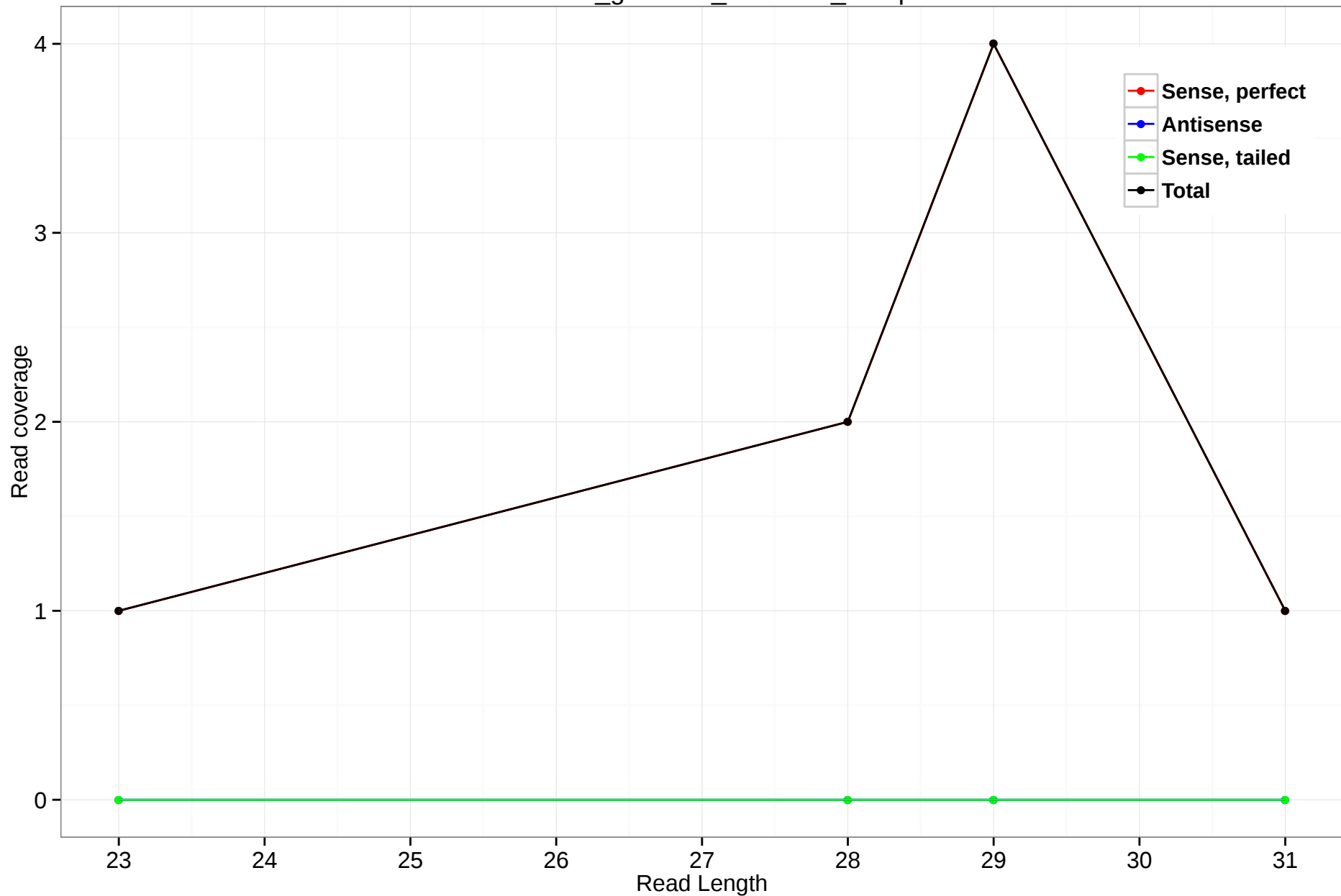
rheMac3_genscan_chr6.808_13.5p
