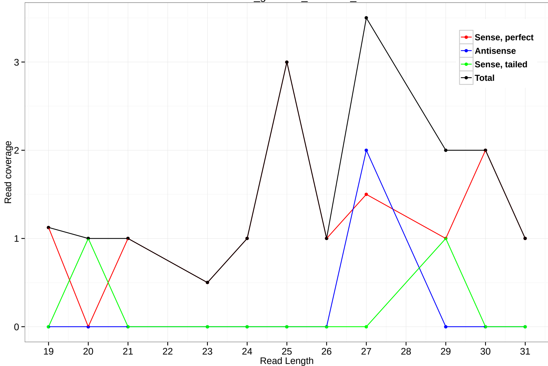
rheMac3_genscan_chr6.799_5
