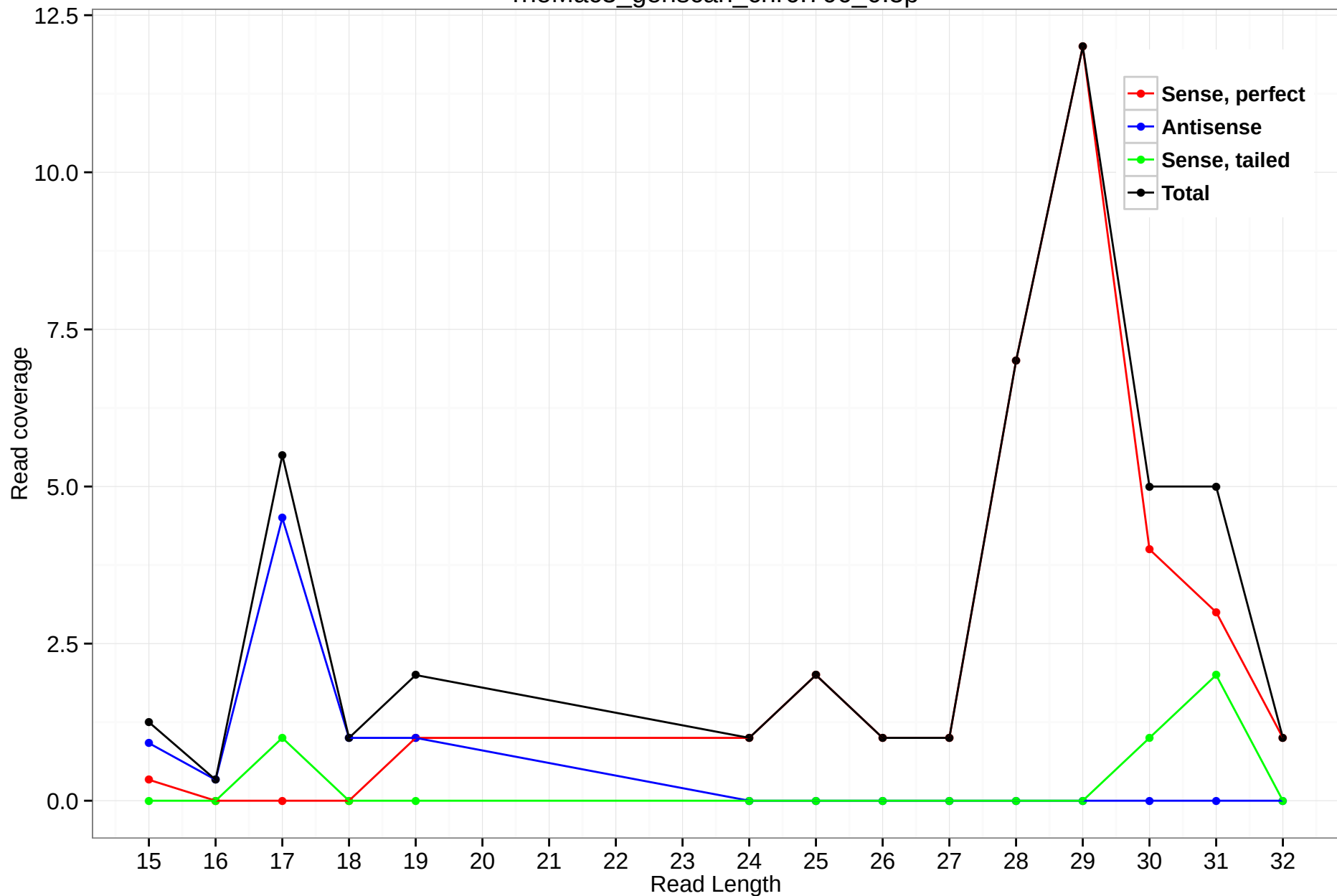
rheMac3_genscan_chr6.706_0.5p
