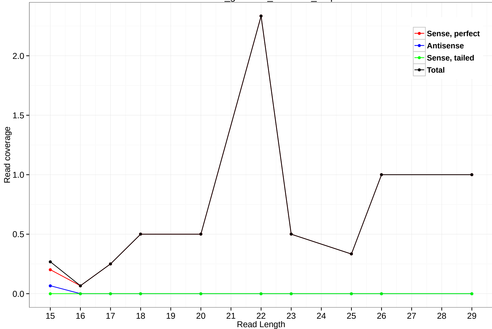
rheMac3_genscan_chr6.698_0.5p
