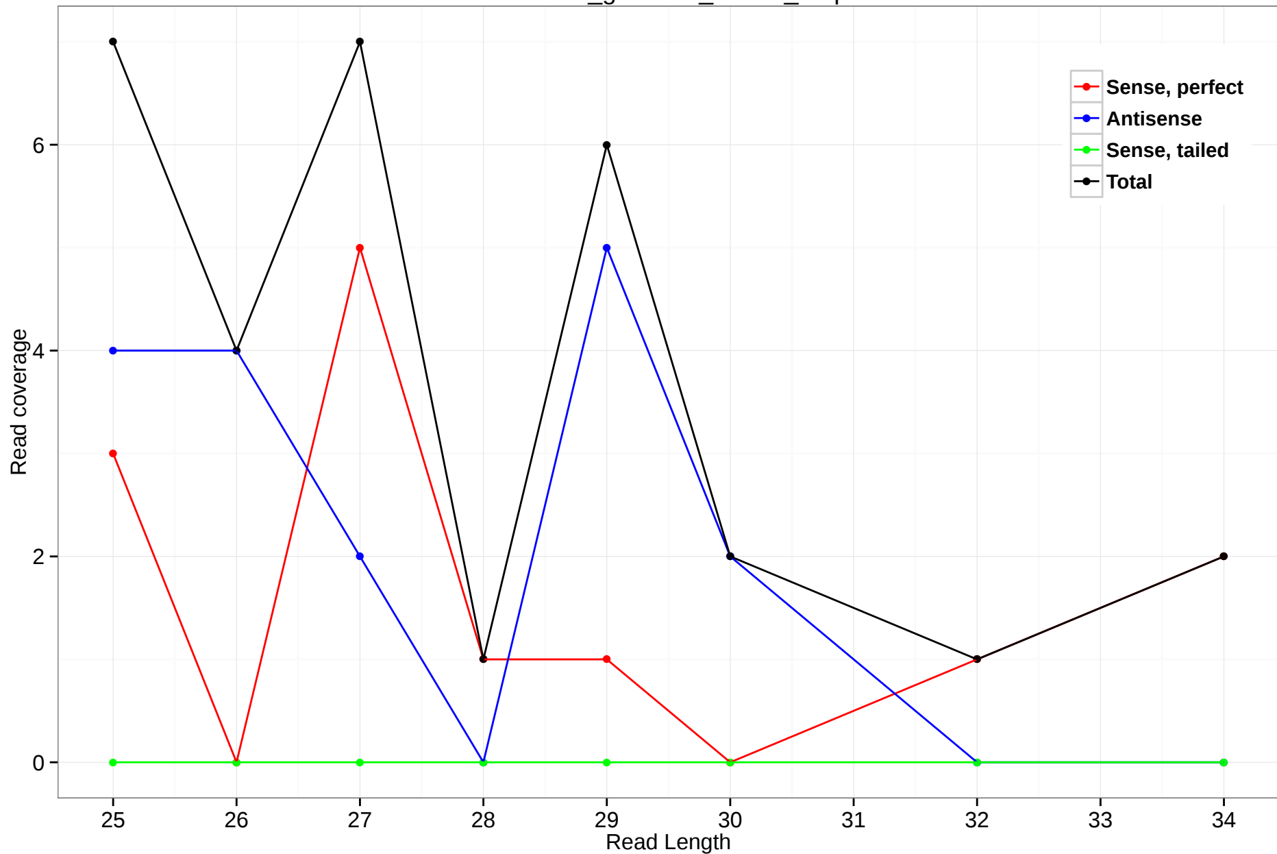
rheMac3_genscan_chr6.5_4.3p
