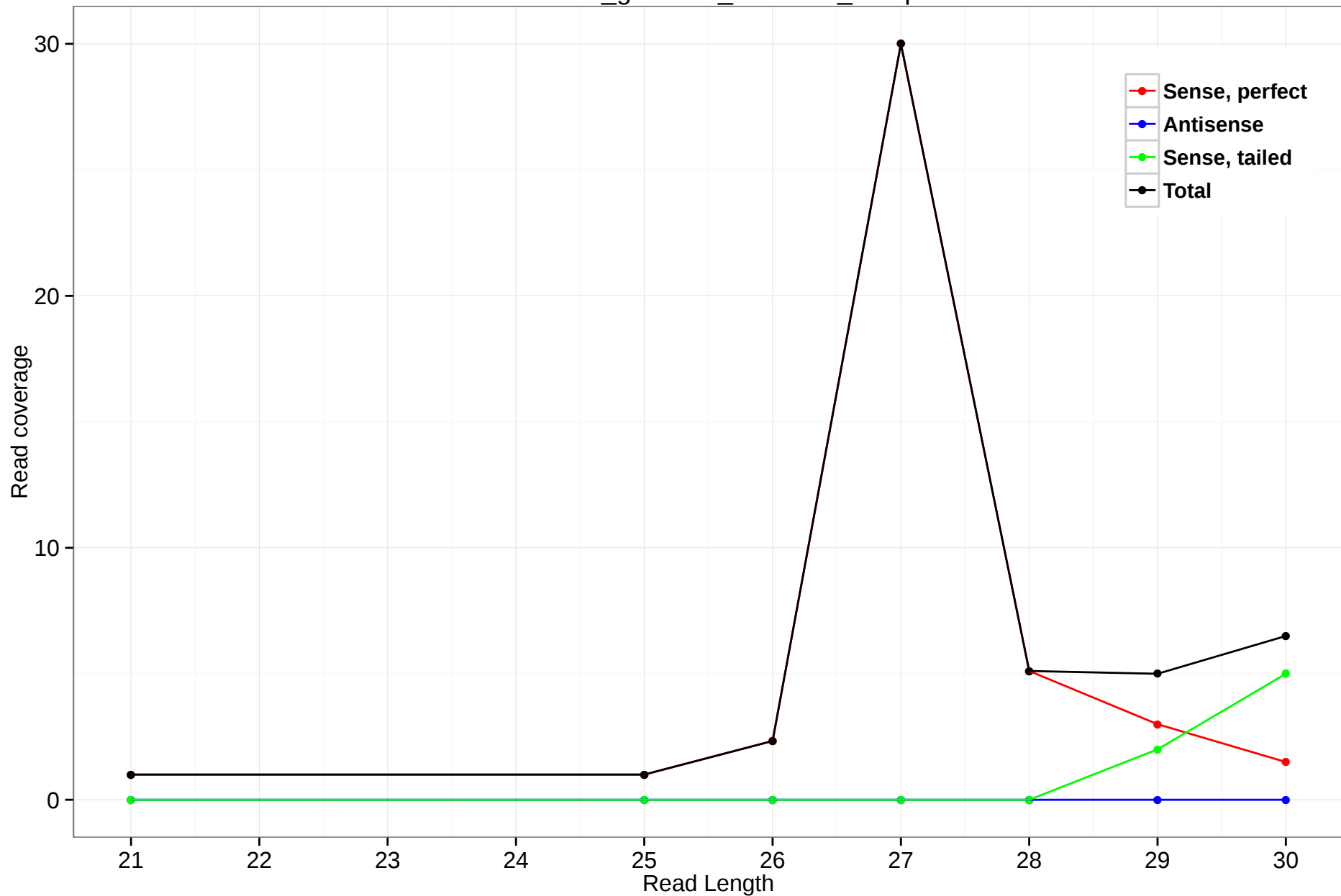
rheMac3_genscan_chr6.577_26.3p
