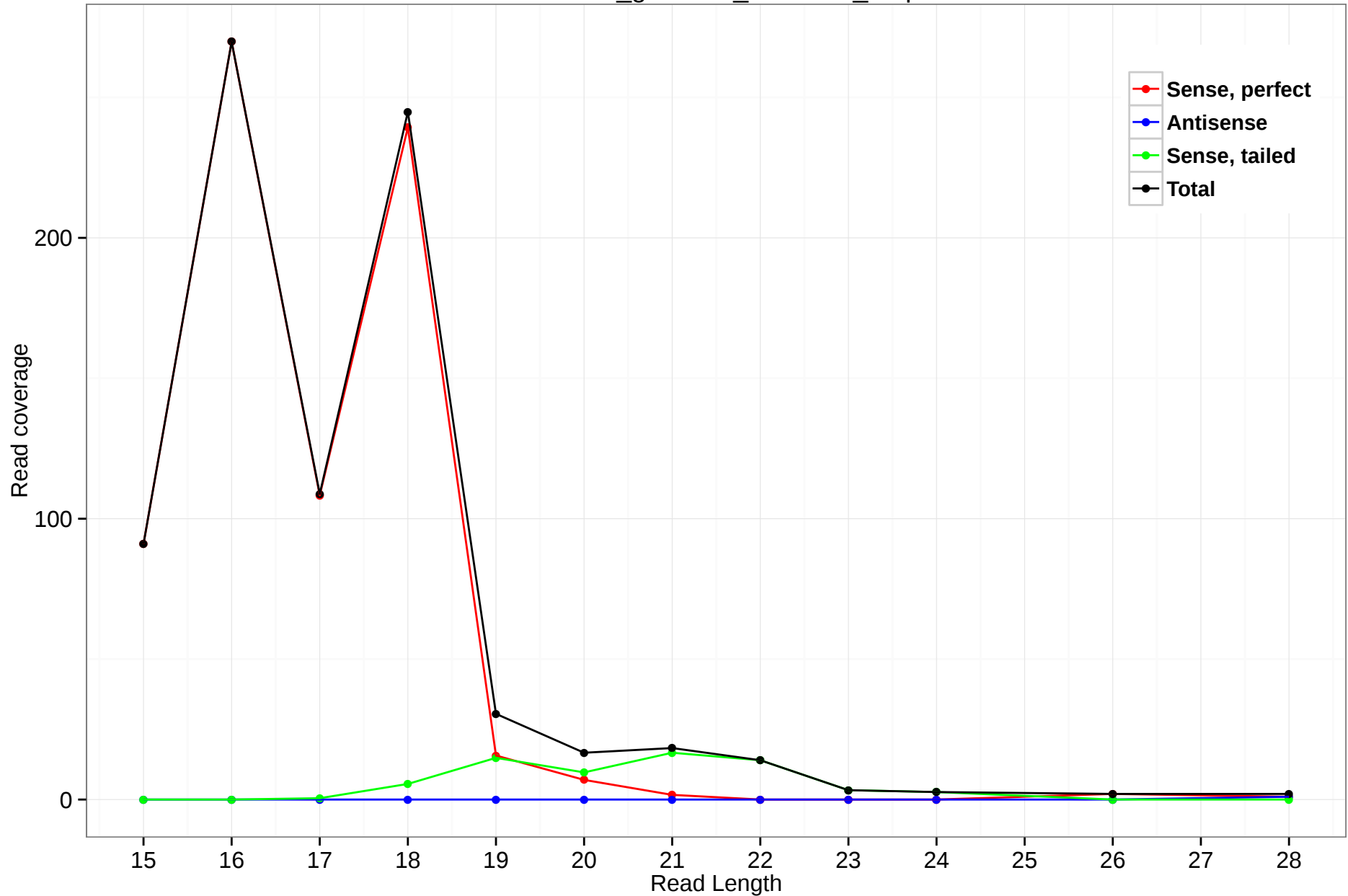
rheMac3_genscan_chr6.419_1.3p
