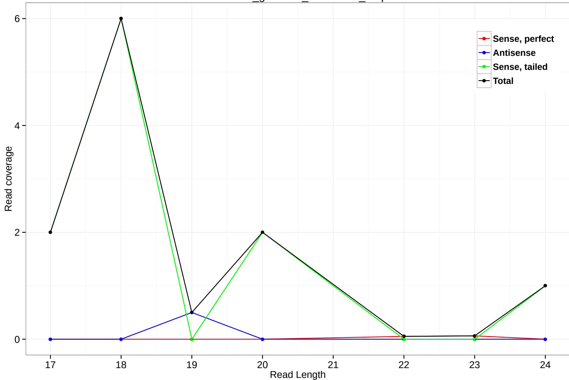
rheMac3_genscan_chr6.3131_3.5p
