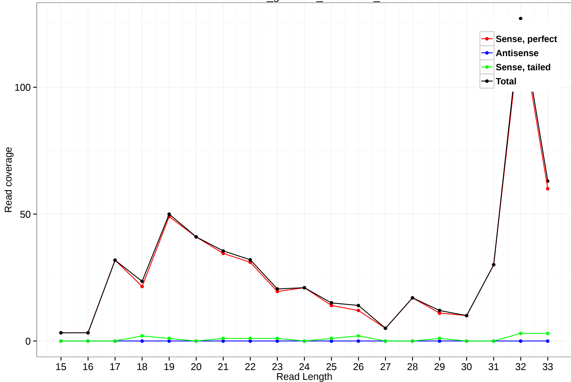
rheMac3_genscan_chr6.3130_8
