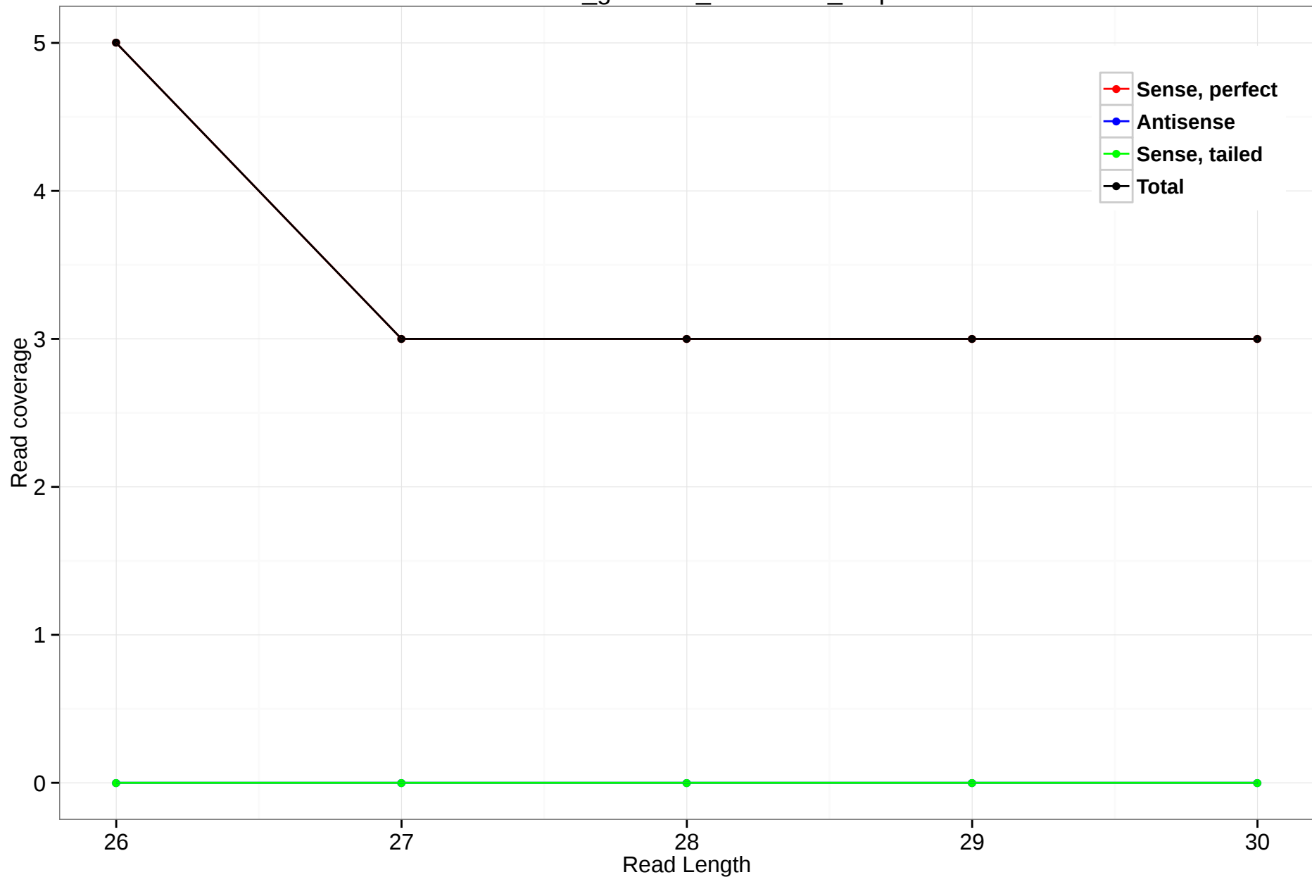
rheMac3_genscan_chr6.3123_2.3p
