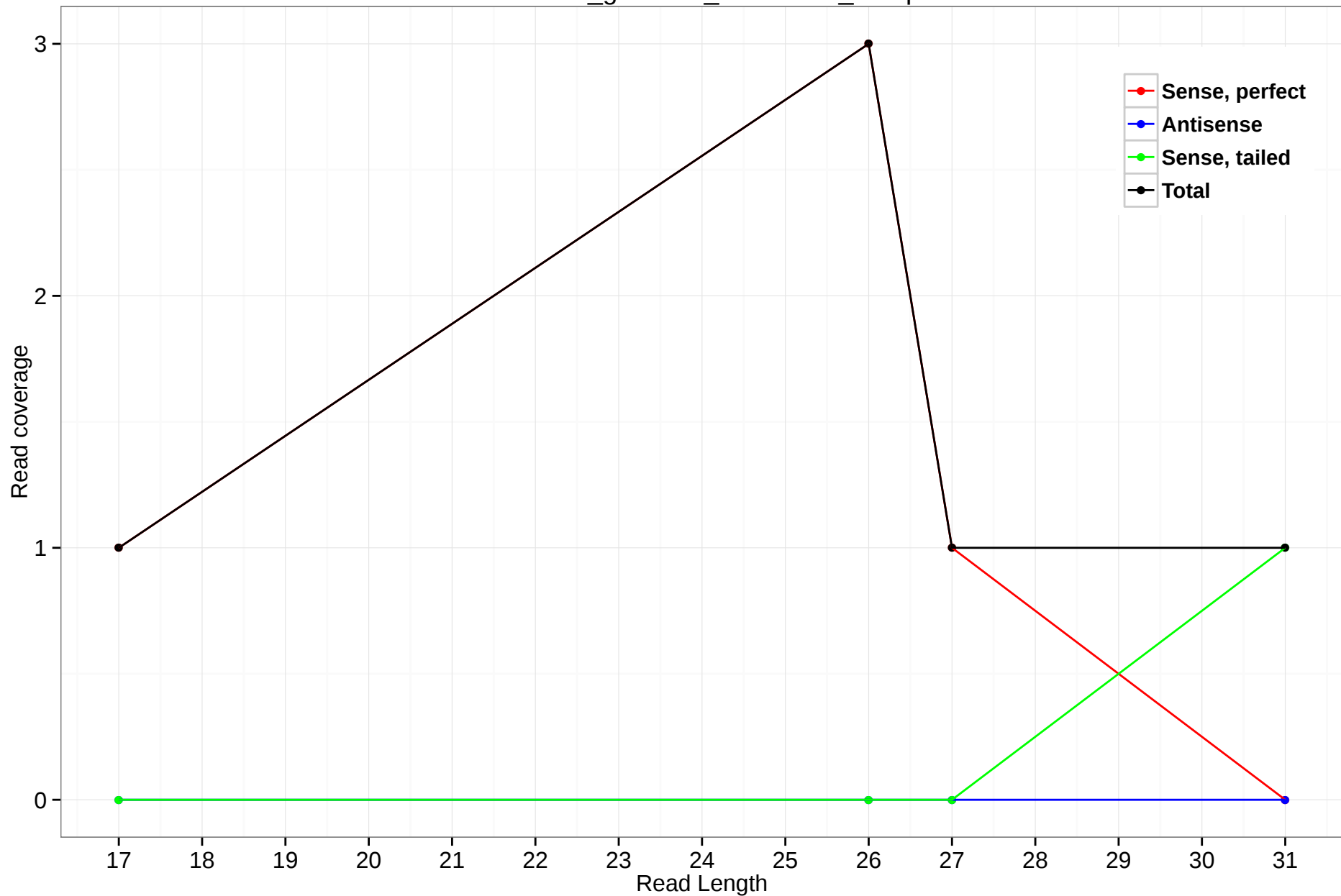
rheMac3_genscan_chr6.3098_20.3p
